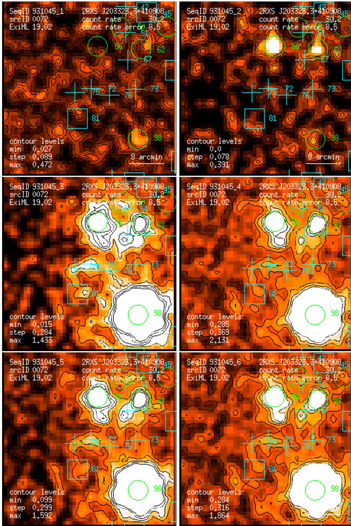
Figure 72: RASS 931045: detection 0072: band rate images, Gaussian filter: (1) PSPC channels 11 – 41, (2) 52 – 90, (3) 91 – 201, (4) 11 – 235, (5) 52 – 201, (6) 11 – 201. Broad band rates in counts/ks. Band rate contour levels in counts/ks/arcmin 2 .
