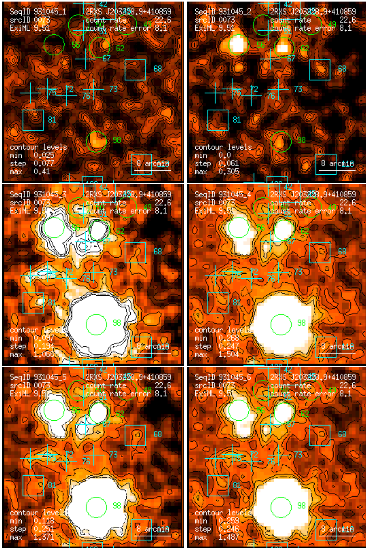
Figure 73: RASS 931045: detection 0073: band rate images, Gaussian filter: (1) PSPC channels 11 – 41, (2) 52 – 90, (3) 91 – 201, (4) 11 – 235, (5) 52 – 201, (6) 11 – 201. Broad band rates in counts/ks. Band rate contour levels in counts/ks/arcmin 2 .
