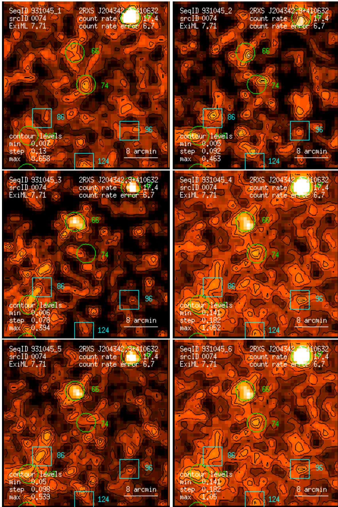
Figure 74: RASS 931045: detection 0074: band rate images, Gaussian filter: (1) PSPC channels 11 – 41, (2) 52 – 90, (3) 91 – 201, (4) 11 – 235, (5) 52 – 201, (6) 11 – 201. Broad band rates in counts/ks. Band rate contour levels in counts/ks/arcmin 2 .
