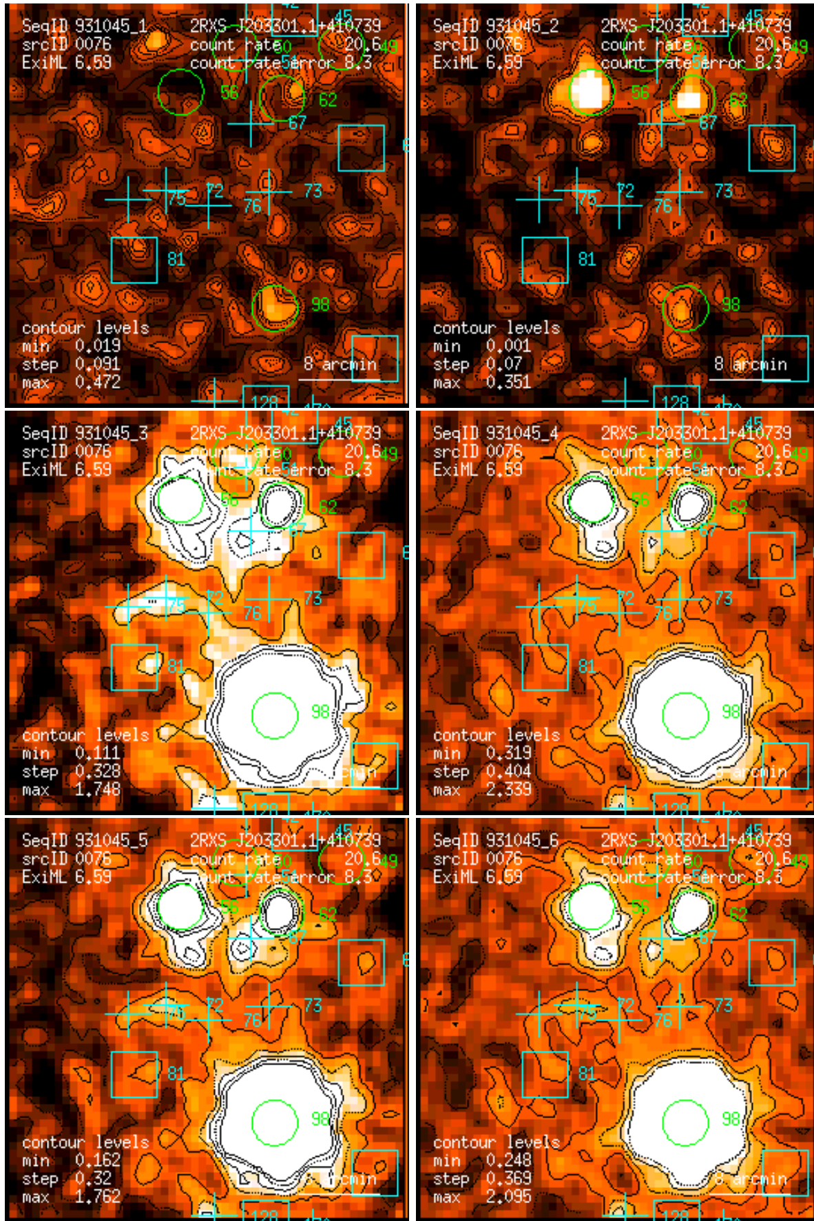
Figure 76: RASS 931045: detection 0076: band rate images, Gaussian filter: (1) PSPC channels 11 – 41, (2) 52 – 90, (3) 91 – 201, (4) 11 – 235, (5) 52 – 201, (6) 11 – 201. Broad band rates in counts/ks. Band rate contour levels in counts/ks/arcmin 2 .
