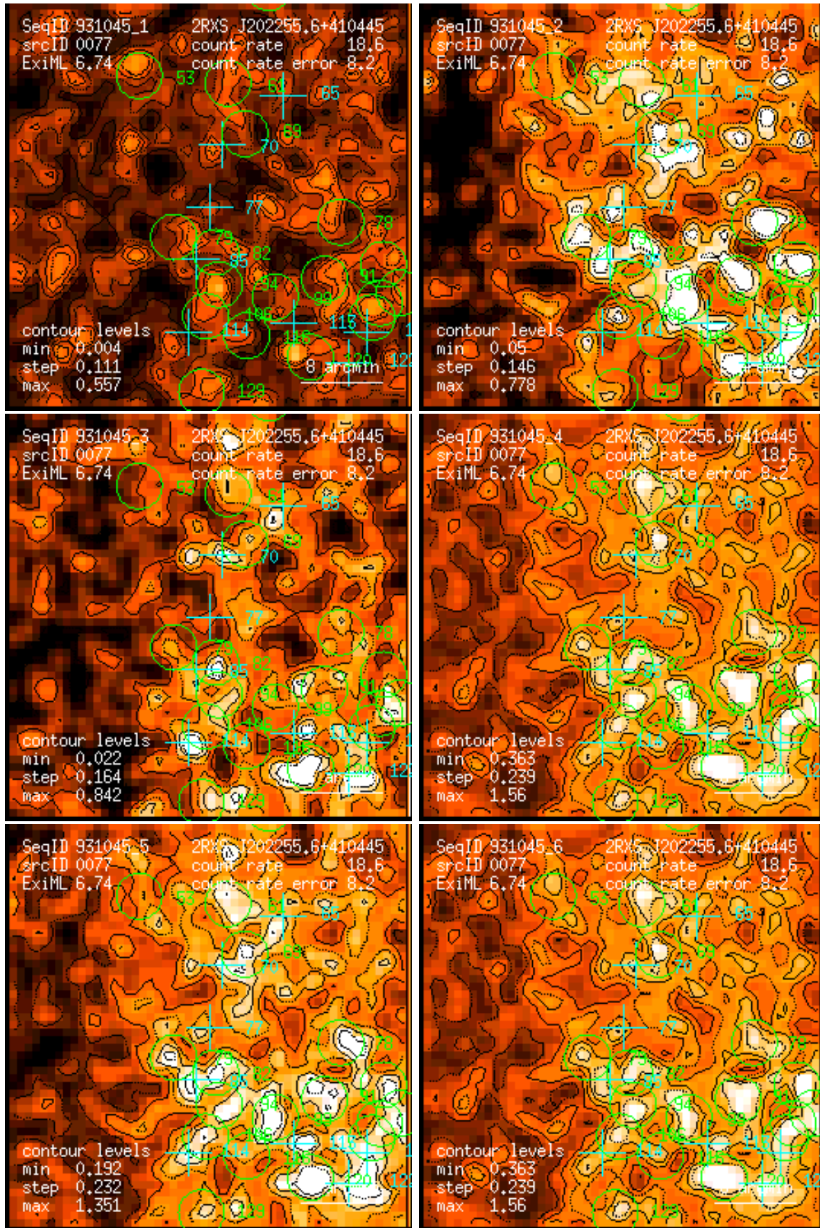
Figure 77: RASS 931045: detection 0077: band rate images, Gaussian filter: (1) PSPC channels 11 – 41, (2) 52 – 90, (3) 91 – 201, (4) 11 – 235, (5) 52 – 201, (6) 11 – 201. Broad band rates in counts/ks. Band rate contour levels in counts/ks/arcmin 2 .
