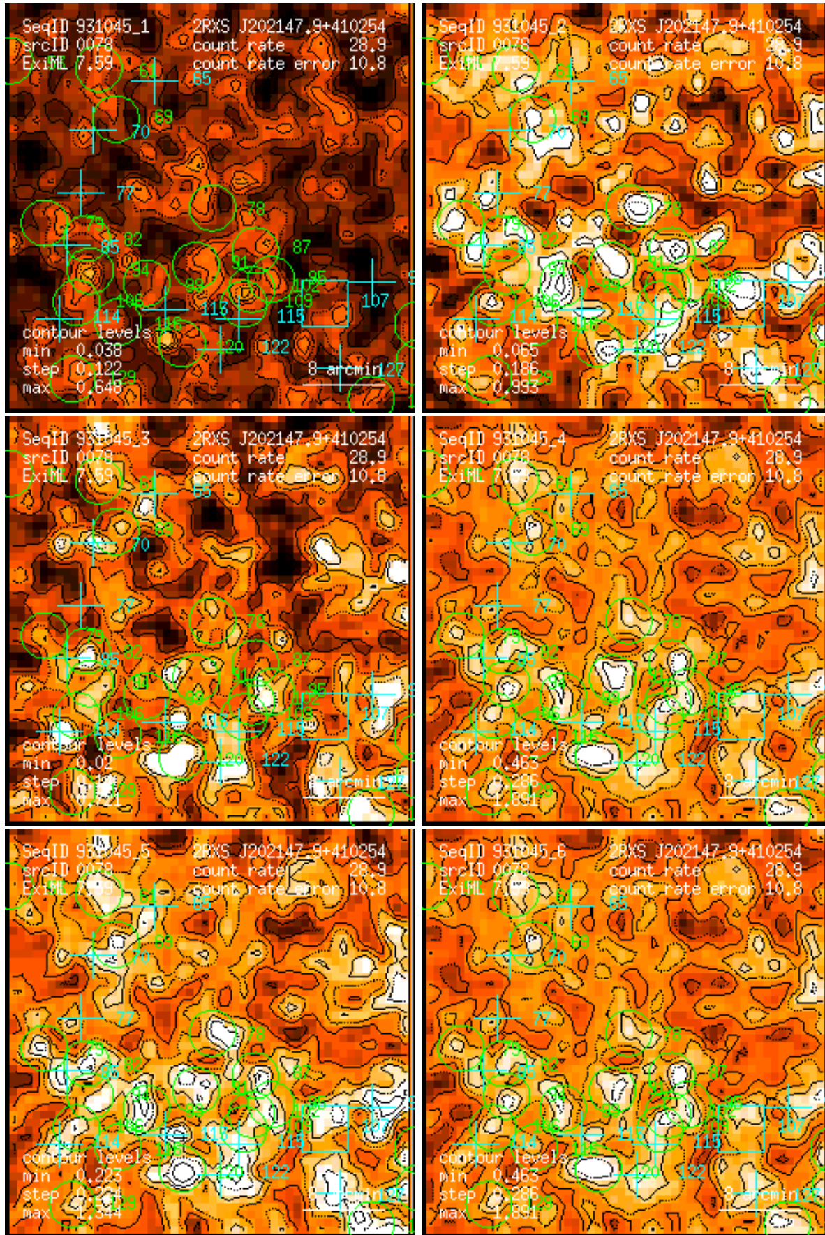
Figure 78: RASS 931045: detection 0078: band rate images, Gaussian filter: (1) PSPC channels 11 – 41, (2) 52 – 90, (3) 91 – 201, (4) 11 – 235, (5) 52 – 201, (6) 11 – 201. Broad band rates in counts/ks. Band rate contour levels in counts/ks/arcmin 2 .
