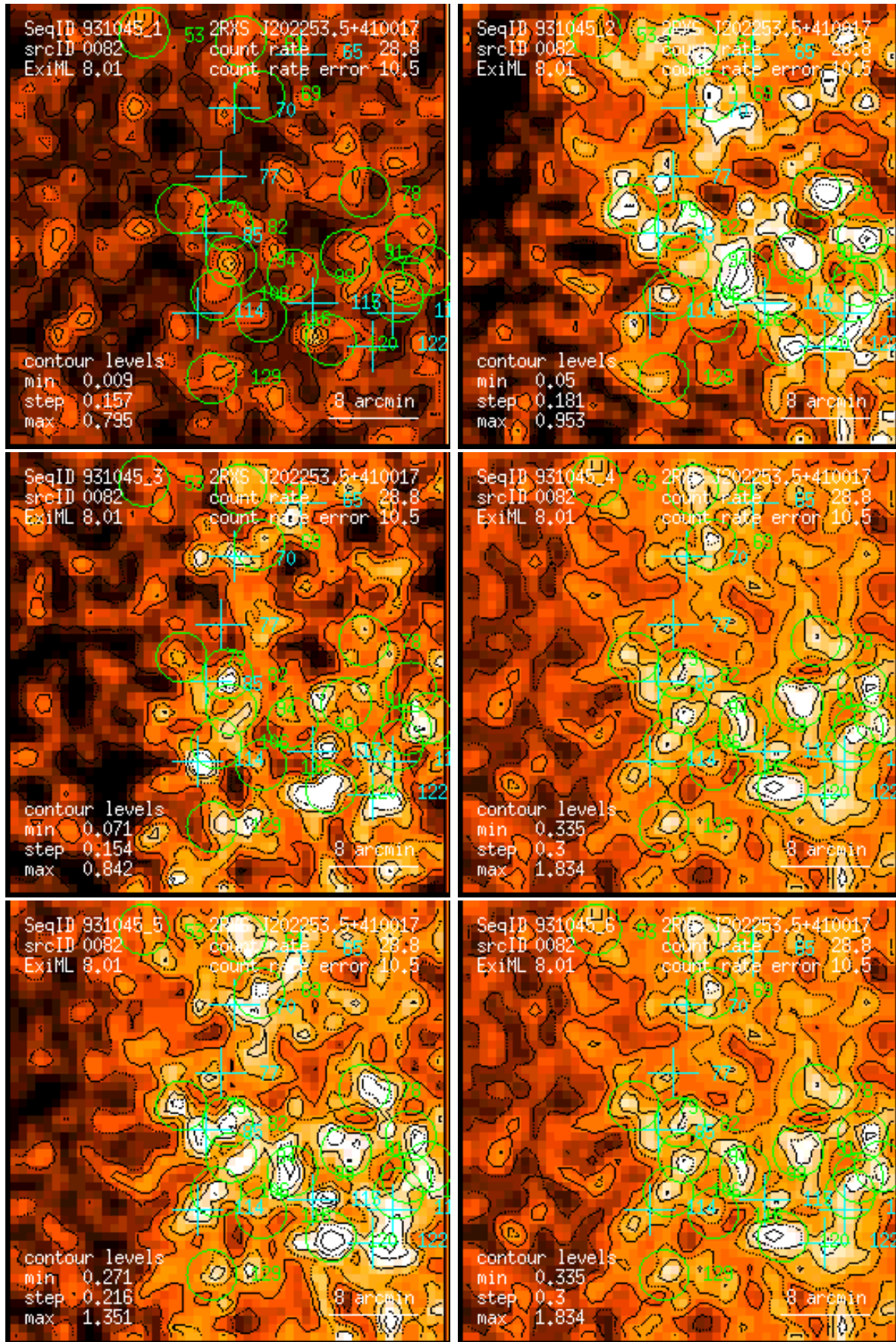
Figure 82: RASS 931045: detection 0082: band rate images, Gaussian filter: (1) PSPC channels 11 – 41, (2) 52 – 90, (3) 91 – 201, (4) 11 – 235, (5) 52 – 201, (6) 11 – 201. Broad band rates in counts/ks. Band rate contour levels in counts/ks/arcmin 2 .
