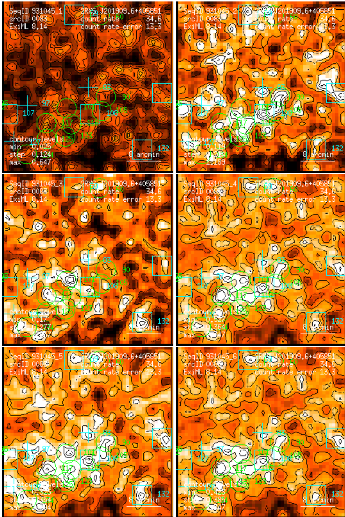
Figure 83: RASS 931045: detection 0083: band rate images, Gaussian filter: (1) PSPC channels 11 – 41, (2) 52 – 90, (3) 91 – 201, (4) 11 – 235, (5) 52 – 201, (6) 11 – 201. Broad band rates in counts/ks. Band rate contour levels in counts/ks/arcmin 2 .
