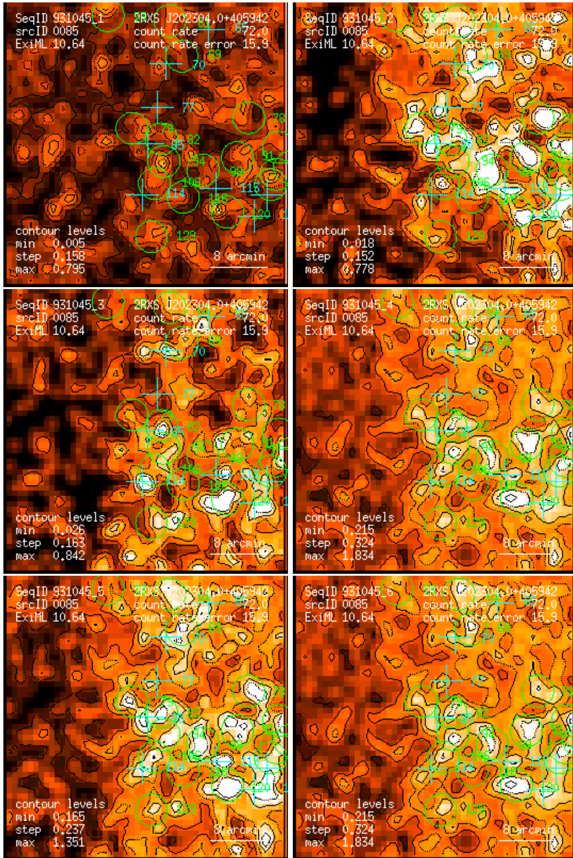
Figure 85: RASS 931045: detection 0085: band rate images, Gaussian filter: (1) PSPC channels 11 – 41, (2) 52 – 90, (3) 91 – 201, (4) 11 – 235, (5) 52 – 201, (6) 11 – 201. Broad band rates in counts/ks. Band rate contour levels in counts/ks/arcmin 2 .
