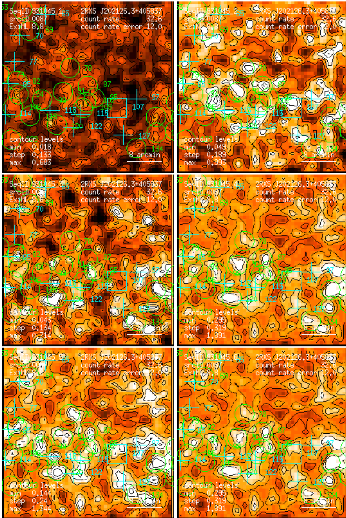
Figure 87: RASS 931045: detection 0087: band rate images, Gaussian filter: (1) PSPC channels 11 – 41, (2) 52 – 90, (3) 91 – 201, (4) 11 – 235, (5) 52 – 201, (6) 11 – 201. Broad band rates in counts/ks. Band rate contour levels in counts/ks/arcmin 2 .
