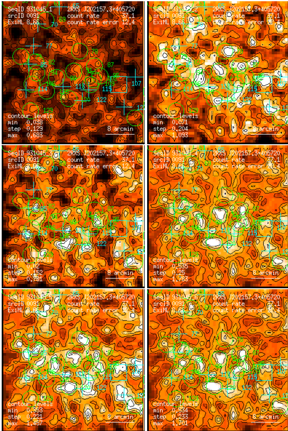
Figure 91: RASS 931045: detection 0091: band rate images, Gaussian filter: (1) PSPC channels 11 – 41, (2) 52 – 90, (3) 91 – 201, (4) 11 – 235, (5) 52 – 201, (6) 11 – 201. Broad band rates in counts/ks. Band rate contour levels in counts/ks/arcmin 2 .
