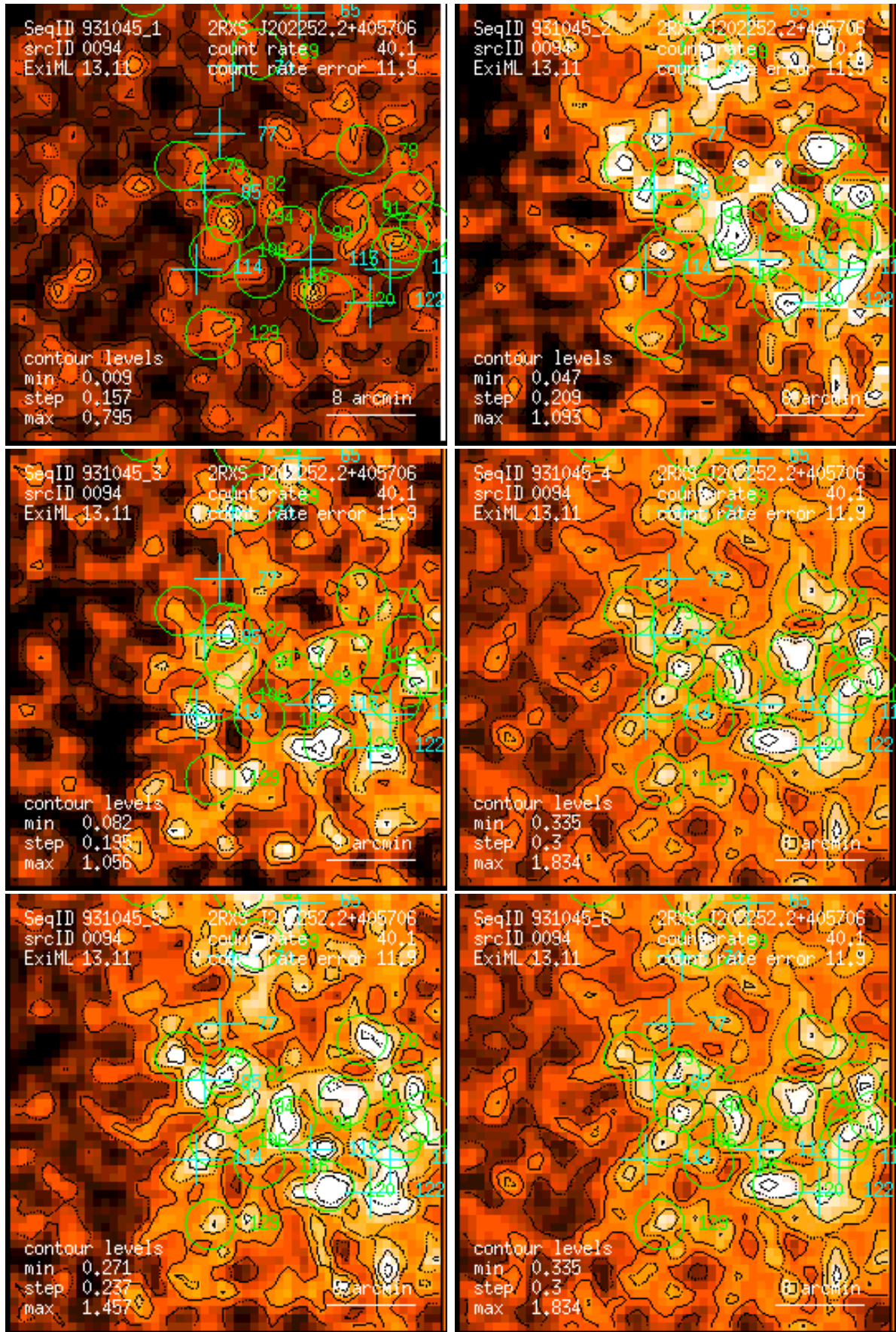
Figure 94: RASS 931045: detection 0094: band rate images, Gaussian filter: (1) PSPC channels 11 – 41, (2) 52 – 90, (3) 91 – 201, (4) 11 – 235, (5) 52 – 201, (6) 11 – 201. Broad band rates in counts/ks. Band rate contour levels in counts/ks/arcmin 2 .
