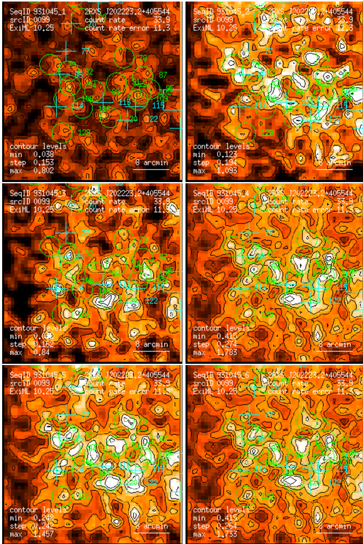
Figure 99: RASS 931045: detection 0099: band rate images, Gaussian filter: (1) PSPC channels 11 – 41, (2) 52 – 90, (3) 91 – 201, (4) 11 – 235, (5) 52 – 201, (6) 11 – 201. Broad band rates in counts/ks. Band rate contour levels in counts/ks/arcmin 2 .
