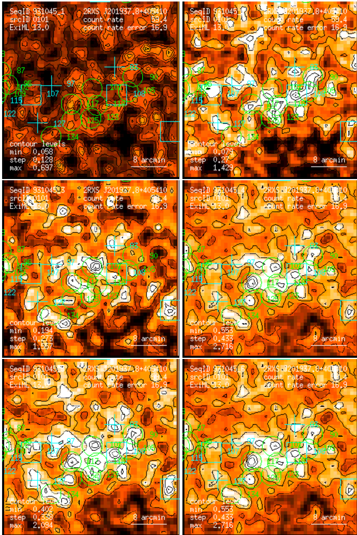
Figure 101: RASS 931045: detection 0101: band rate images, Gaussian filter: (1) PSPC channels 11 – 41, (2) 52 – 90, (3) 91 – 201, (4) 11 – 235, (5) 52 – 201, (6) 11 – 201. Broad band rates in counts/ks. Band rate contour levels in counts/ks/arcmin 2 .
