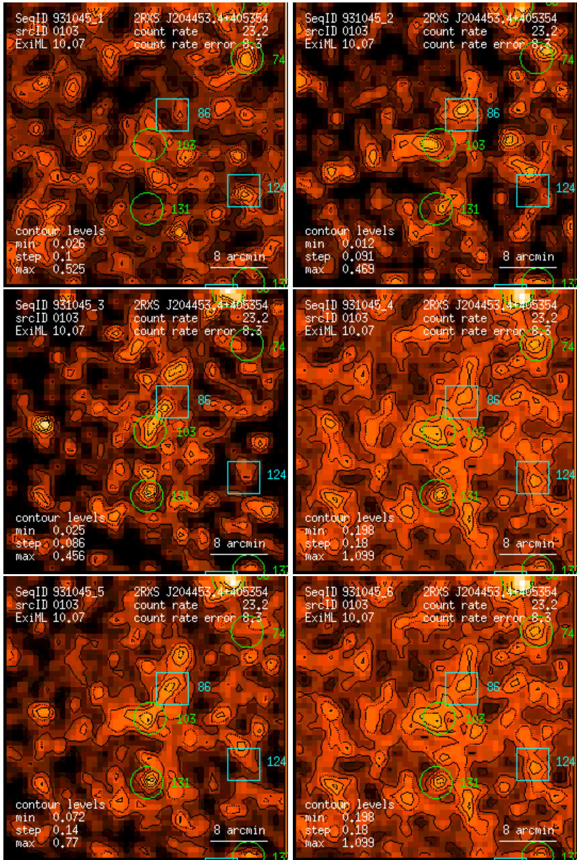
Figure 103: RASS 931045: detection 0103: band rate images, Gaussian filter: (1) PSPC channels 11 – 41, (2) 52 – 90, (3) 91 – 201, (4) 11 – 235, (5) 52 – 201, (6) 11 – 201. Broad band rates in counts/ks. Band rate contour levels in counts/ks/arcmin 2 .
