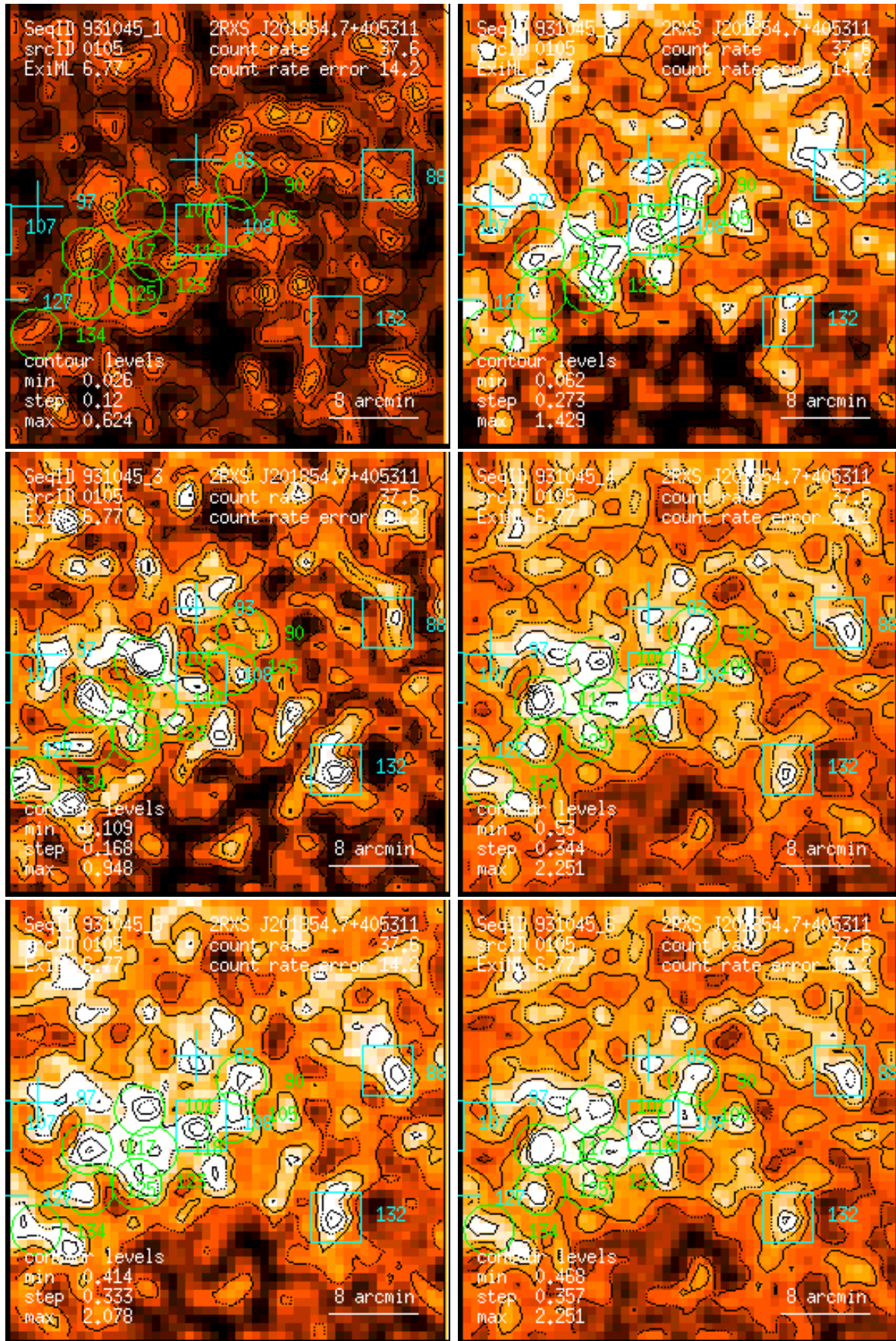
Figure 105: RASS 931045: detection 0105: band rate images, Gaussian filter: (1) PSPC channels 11 – 41, (2) 52 – 90, (3) 91 – 201, (4) 11 – 235, (5) 52 – 201, (6) 11 – 201. Broad band rates in counts/ks. Band rate contour levels in counts/ks/arcmin 2 .
