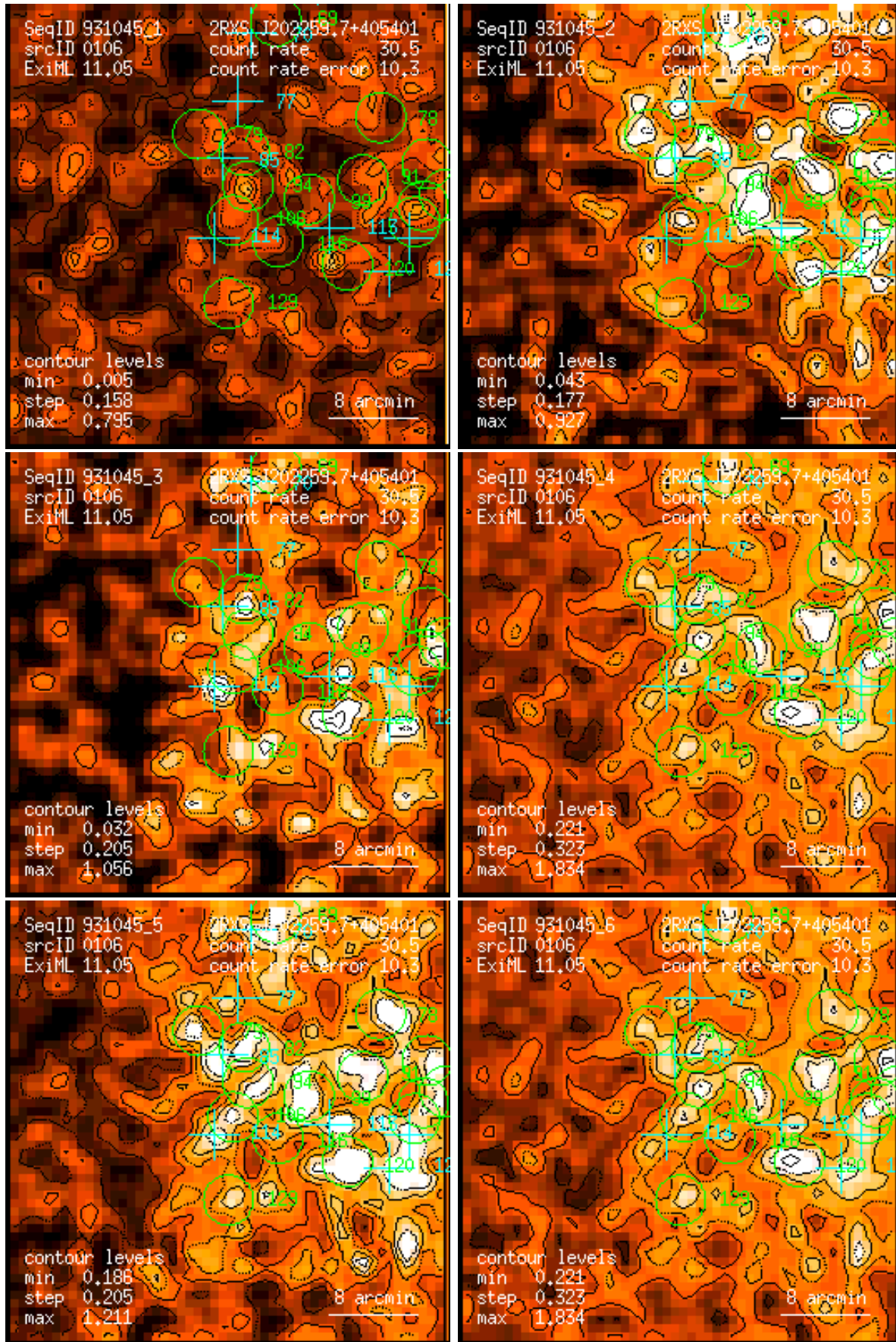
Figure 106: RASS 931045: detection 0106: band rate images, Gaussian filter: (1) PSPC channels 11 – 41, (2) 52 – 90, (3) 91 – 201, (4) 11 – 235, (5) 52 – 201, (6) 11 – 201. Broad band rates in counts/ks. Band rate contour levels in counts/ks/arcmin 2 .
