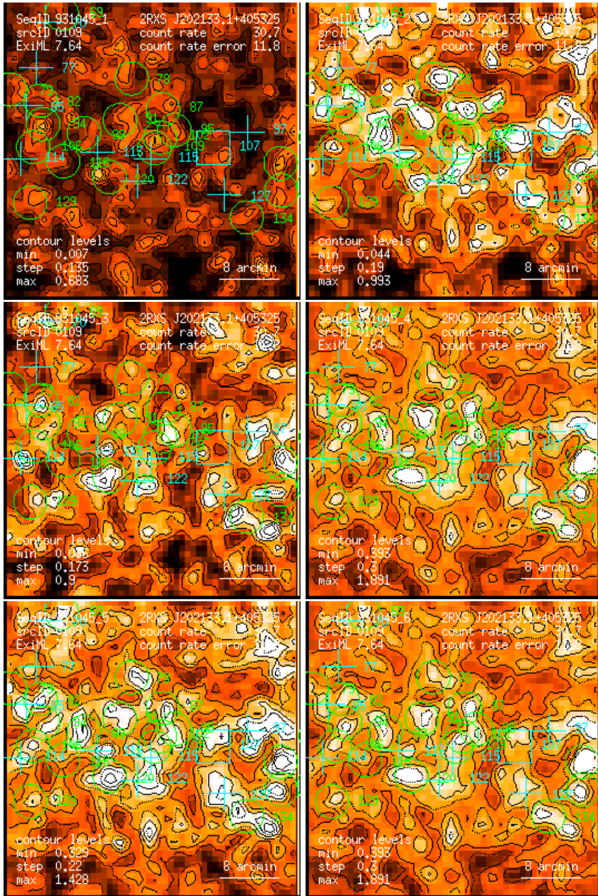
Figure 109: RASS 931045: detection 0109: band rate images, Gaussian filter: (1) PSPC channels 11 – 41, (2) 52 – 90, (3) 91 – 201, (4) 11 – 235, (5) 52 – 201, (6) 11 – 201. Broad band rates in counts/ks. Band rate contour levels in counts/ks/arcmin 2 .
