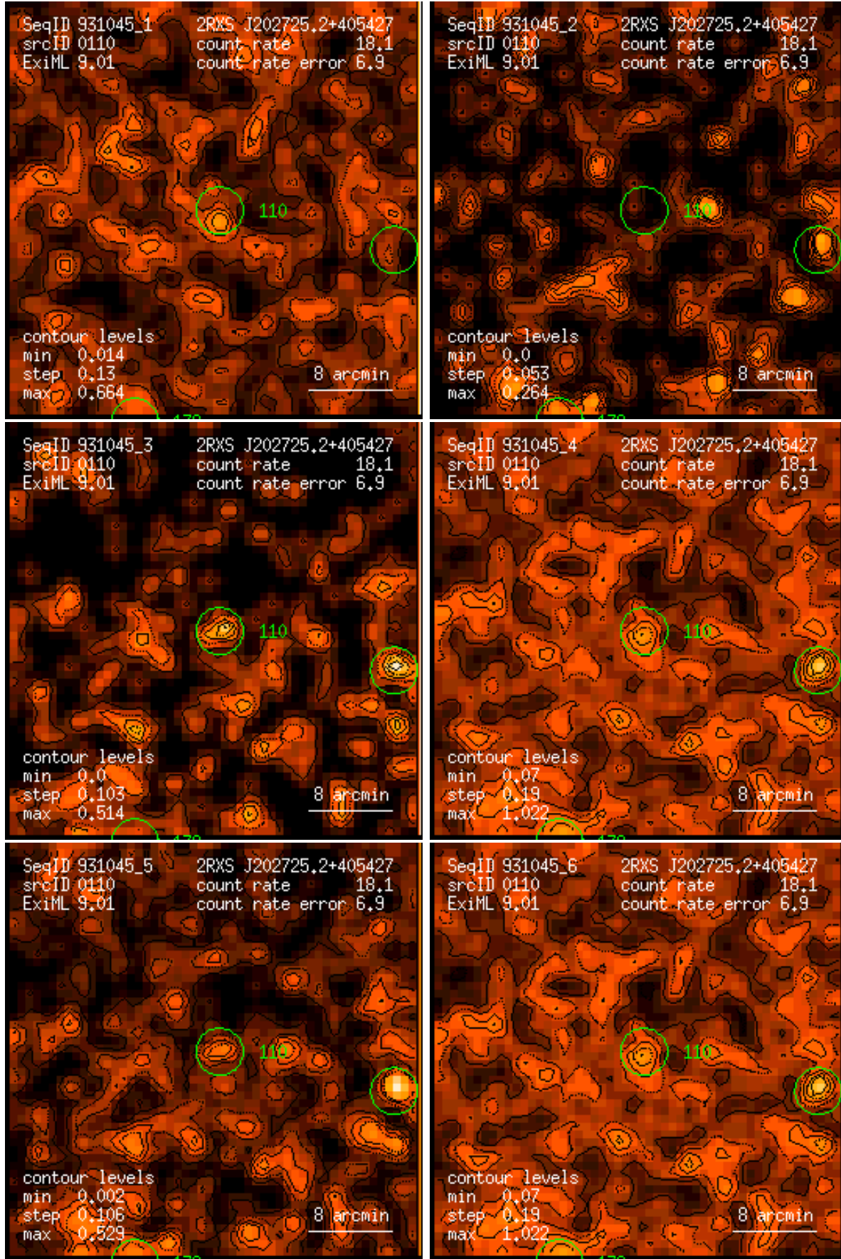
Figure 110: RASS 931045: detection 0110: band rate images, Gaussian filter: (1) PSPC channels 11 – 41, (2) 52 – 90, (3) 91 – 201, (4) 11 – 235, (5) 52 – 201, (6) 11 – 201. Broad band rates in counts/ks. Band rate contour levels in counts/ks/arcmin 2 .
