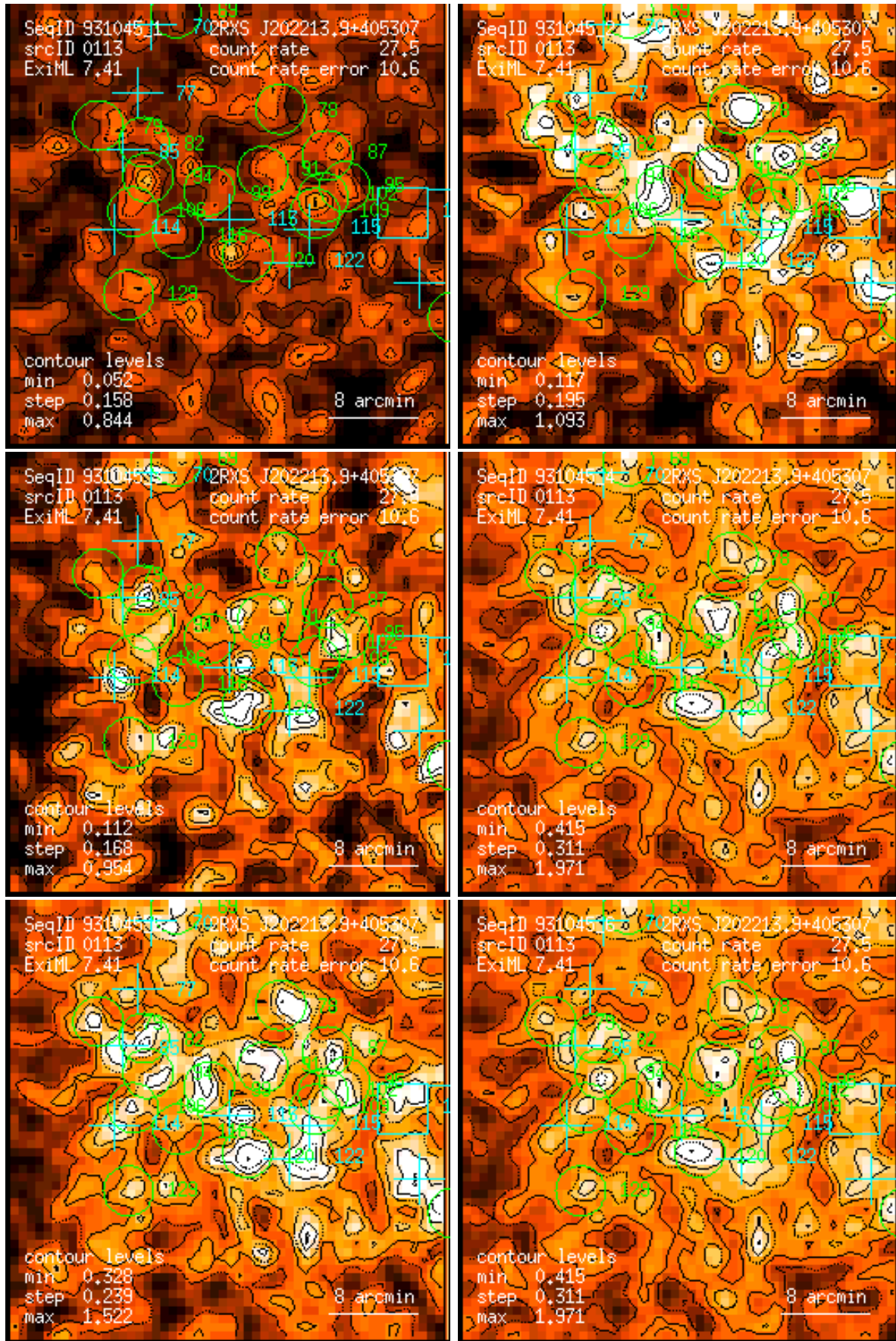
Figure 113: RASS 931045: detection 0113: band rate images, Gaussian filter: (1) PSPC channels 11 – 41, (2) 52 – 90, (3) 91 – 201, (4) 11 – 235, (5) 52 – 201, (6) 11 – 201. Broad band rates in counts/ks. Band rate contour levels in counts/ks/arcmin 2 .
