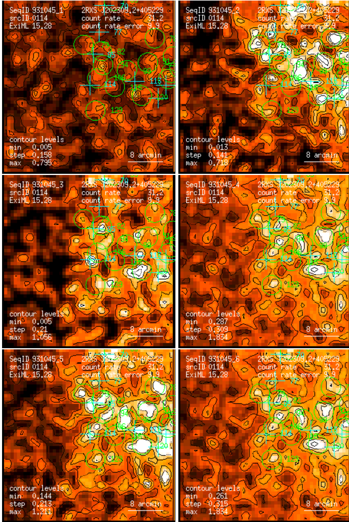
Figure 114: RASS 931045: detection 0114: band rate images, Gaussian filter: (1) PSPC channels 11 – 41, (2) 52 – 90, (3) 91 – 201, (4) 11 – 235, (5) 52 – 201, (6) 11 – 201. Broad band rates in counts/ks. Band rate contour levels in counts/ks/arcmin 2 .
