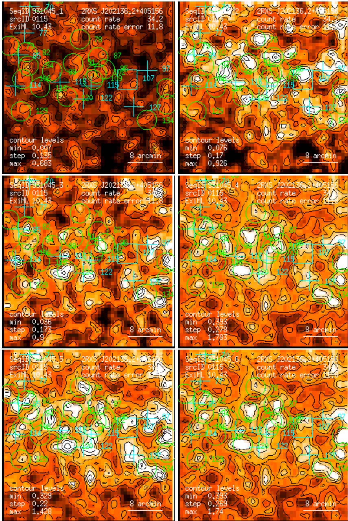
Figure 115: RASS 931045: detection 0115: band rate images, Gaussian filter: (1) PSPC channels 11 – 41, (2) 52 – 90, (3) 91 – 201, (4) 11 – 235, (5) 52 – 201, (6) 11 – 201. Broad band rates in counts/ks. Band rate contour levels in counts/ks/arcmin 2 .
