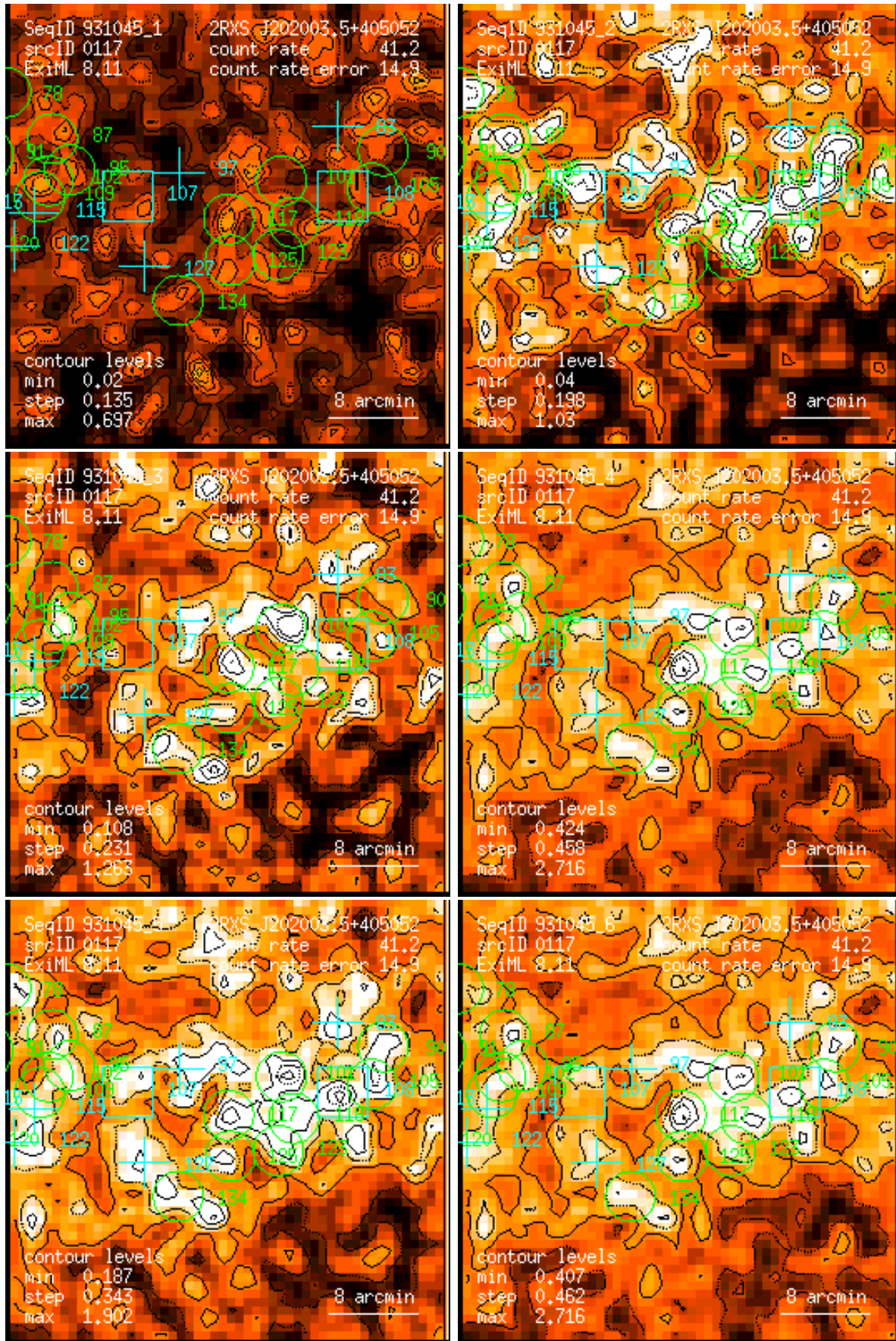
Figure 117: RASS 931045: detection 0117: band rate images, Gaussian filter: (1) PSPC channels 11 – 41, (2) 52 – 90, (3) 91 – 201, (4) 11 – 235, (5) 52 – 201, (6) 11 – 201. Broad band rates in counts/ks. Band rate contour levels in counts/ks/arcmin 2 .
