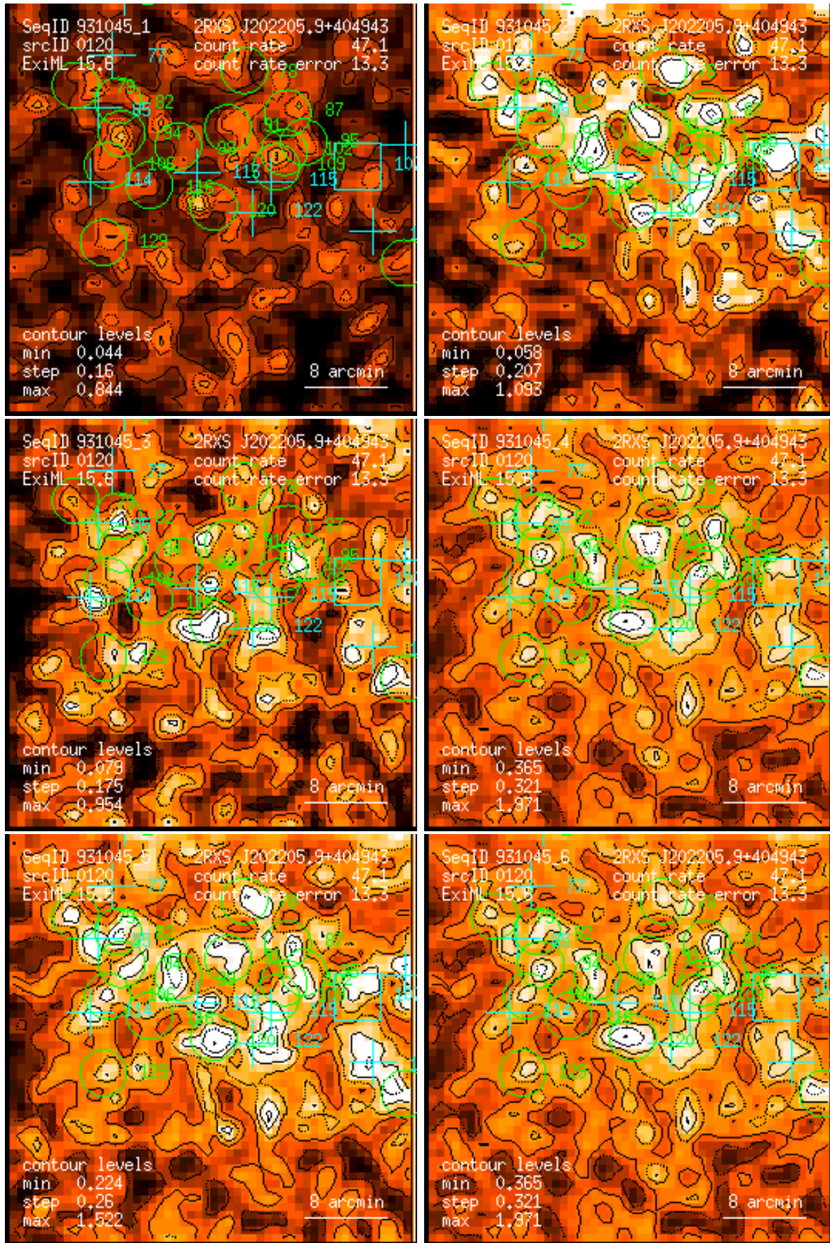
Figure 120: RASS 931045: detection 0120: band rate images, Gaussian filter: (1) PSPC channels 11 – 41, (2) 52 – 90, (3) 91 – 201, (4) 11 – 235, (5) 52 – 201, (6) 11 – 201. Broad band rates in counts/ks. Band rate contour levels in counts/ks/arcmin 2 .
