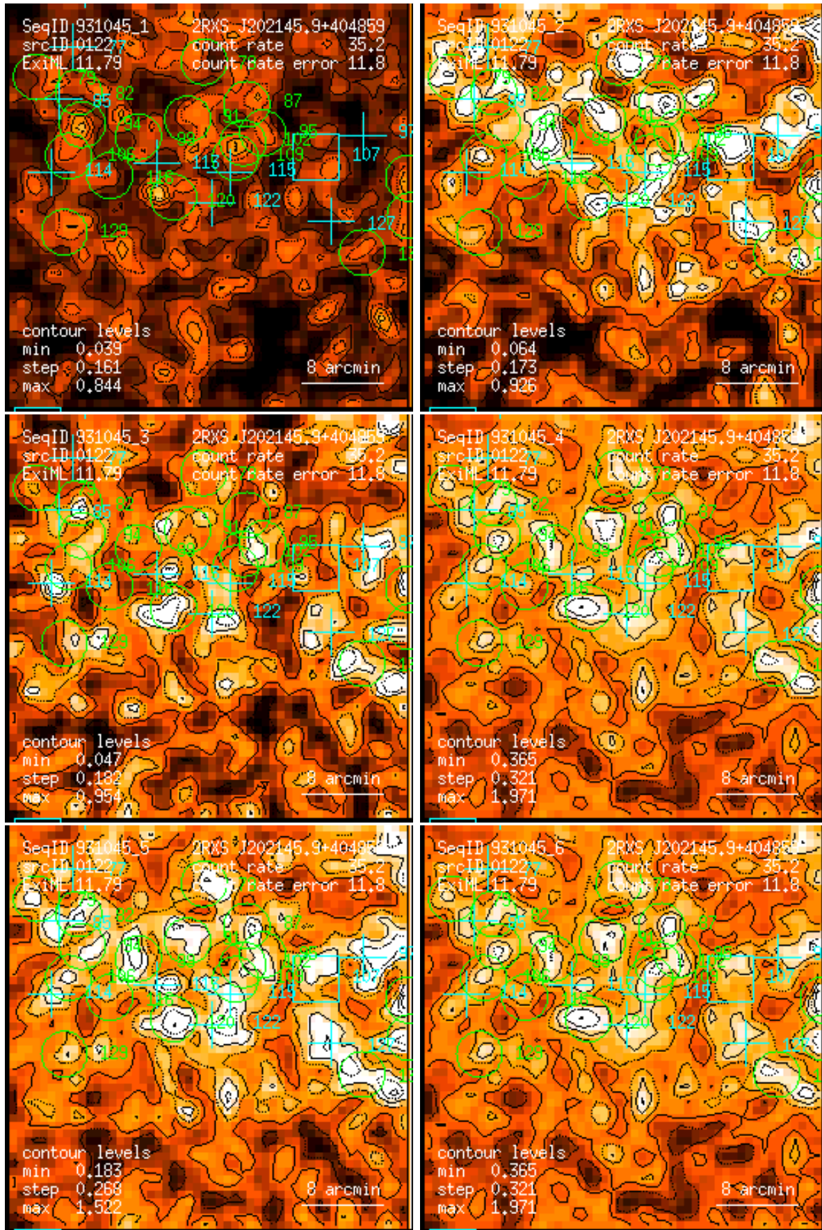
Figure 122: RASS 931045: detection 0122: band rate images, Gaussian filter: (1) PSPC channels 11 – 41, (2) 52 – 90, (3) 91 – 201, (4) 11 – 235, (5) 52 – 201, (6) 11 – 201. Broad band rates in counts/ks. Band rate contour levels in counts/ks/arcmin 2 .
