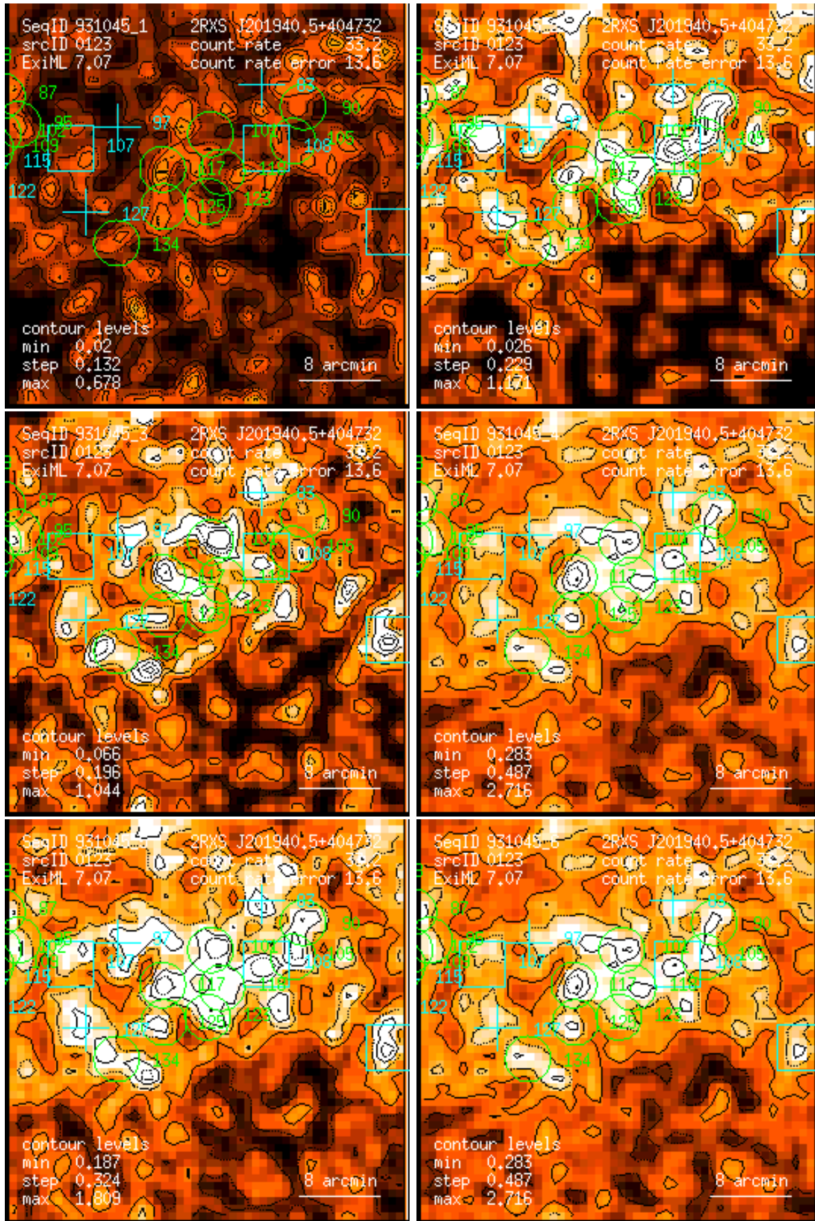
Figure 123: RASS 931045: detection 0123: band rate images, Gaussian filter: (1) PSPC channels 11 – 41, (2) 52 – 90, (3) 91 – 201, (4) 11 – 235, (5) 52 – 201, (6) 11 – 201. Broad band rates in counts/ks. Band rate contour levels in counts/ks/arcmin 2 .
