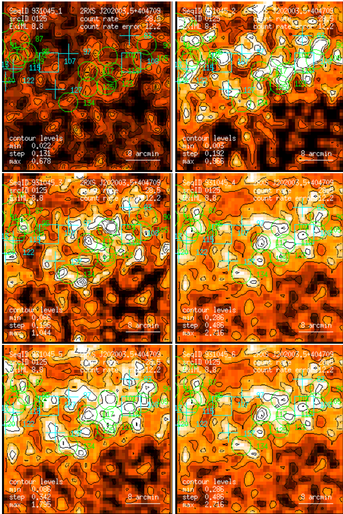
Figure 125: RASS 931045: detection 0125: band rate images, Gaussian filter: (1) PSPC channels 11 – 41, (2) 52 – 90, (3) 91 – 201, (4) 11 – 235, (5) 52 – 201, (6) 11 – 201. Broad band rates in counts/ks. Band rate contour levels in counts/ks/arcmin 2 .
