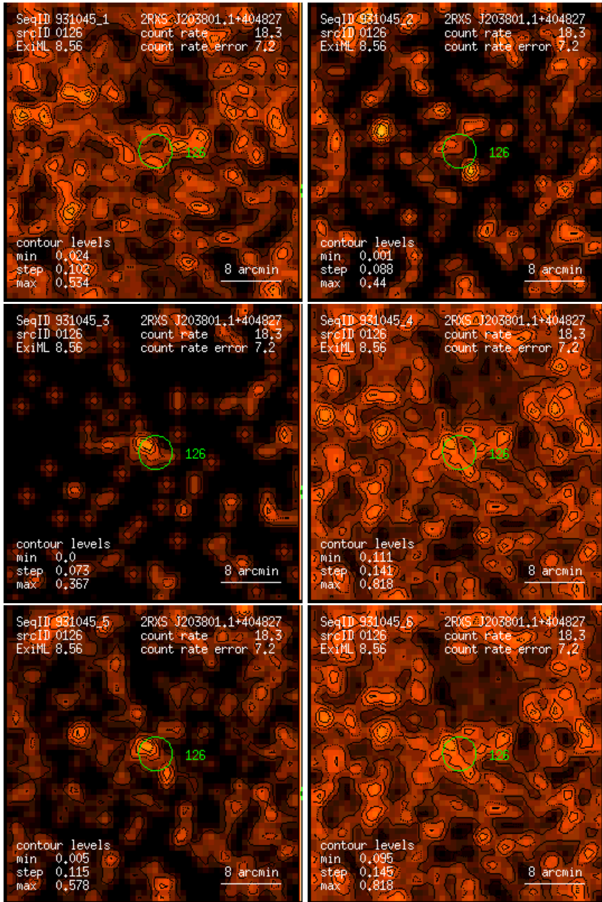
Figure 126: RASS 931045: detection 0126: band rate images, Gaussian filter: (1) PSPC channels 11 – 41, (2) 52 – 90, (3) 91 – 201, (4) 11 – 235, (5) 52 – 201, (6) 11 – 201. Broad band rates in counts/ks. Band rate contour levels in counts/ks/arcmin 2 .
