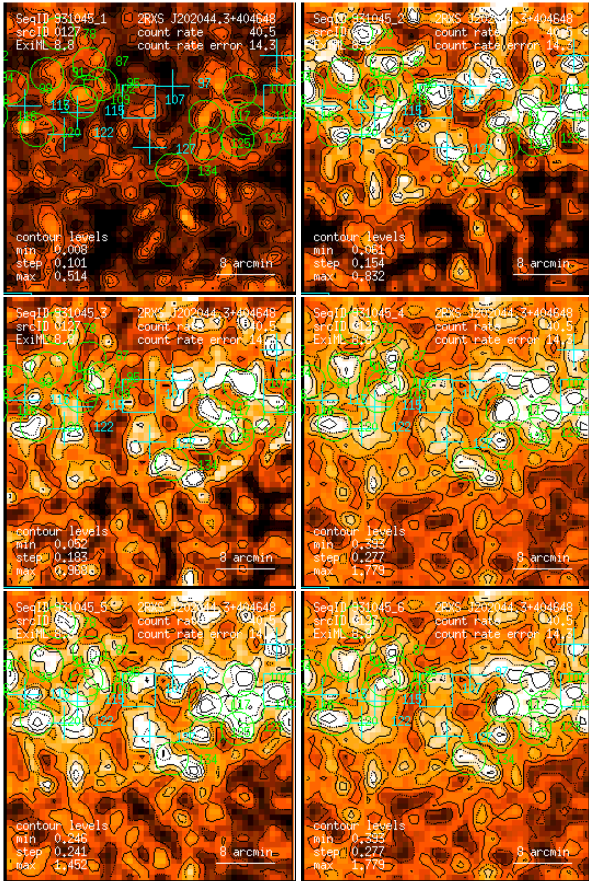
Figure 127: RASS 931045: detection 0127: band rate images, Gaussian filter: (1) PSPC channels 11 – 41, (2) 52 – 90, (3) 91 – 201, (4) 11 – 235, (5) 52 – 201, (6) 11 – 201. Broad band rates in counts/ks. Band rate contour levels in counts/ks/arcmin 2 .
