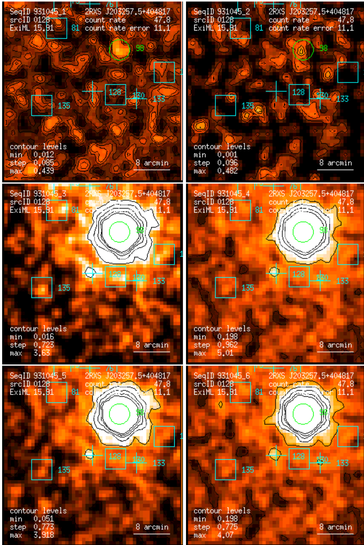
Figure 128: RASS 931045: detection 0128: band rate images, Gaussian filter: (1) PSPC channels 11 – 41, (2) 52 – 90, (3) 91 – 201, (4) 11 – 235, (5) 52 – 201, (6) 11 – 201. Broad band rates in counts/ks. Band rate contour levels in counts/ks/arcmin 2 .
