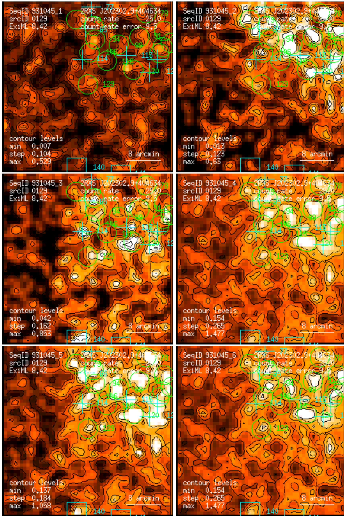
Figure 129: RASS 931045: detection 0129: band rate images, Gaussian filter: (1) PSPC channels 11 – 41, (2) 52 – 90, (3) 91 – 201, (4) 11 – 235, (5) 52 – 201, (6) 11 – 201. Broad band rates in counts/ks. Band rate contour levels in counts/ks/arcmin 2 .
