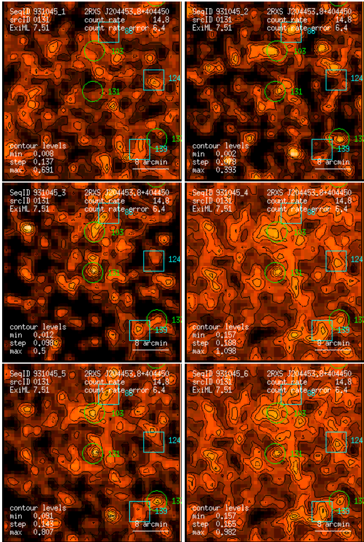
Figure 131: RASS 931045: detection 0131: band rate images, Gaussian filter: (1) PSPC channels 11 – 41, (2) 52 – 90, (3) 91 – 201, (4) 11 – 235, (5) 52 – 201, (6) 11 – 201. Broad band rates in counts/ks. Band rate contour levels in counts/ks/arcmin 2 .
