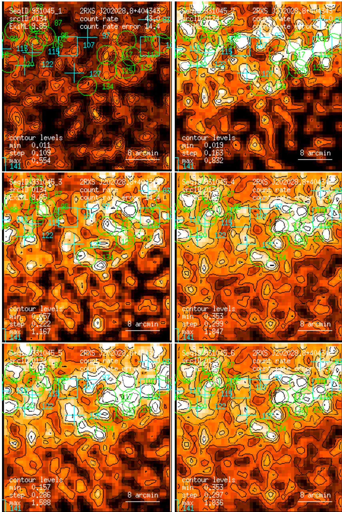
Figure 134: RASS 931045: detection 0134: band rate images, Gaussian filter: (1) PSPC channels 11 – 41, (2) 52 – 90, (3) 91 – 201, (4) 11 – 235, (5) 52 – 201, (6) 11 – 201. Broad band rates in counts/ks. Band rate contour levels in counts/ks/arcmin 2 .
