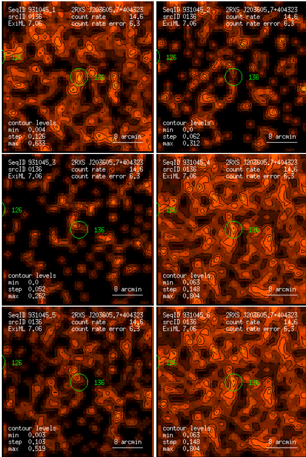
Figure 136: RASS 931045: detection 0136: band rate images, Gaussian filter: (1) PSPC channels 11 – 41, (2) 52 – 90, (3) 91 – 201, (4) 11 – 235, (5) 52 – 201, (6) 11 – 201. Broad band rates in counts/ks. Band rate contour levels in counts/ks/arcmin 2 .
