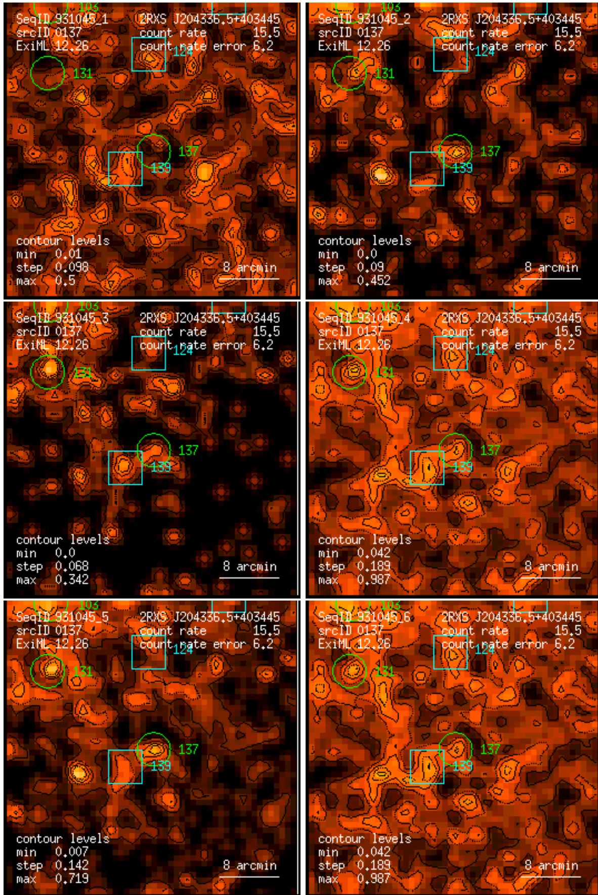
Figure 137: RASS 931045: detection 0137: band rate images, Gaussian filter: (1) PSPC channels 11 – 41, (2) 52 – 90, (3) 91 – 201, (4) 11 – 235, (5) 52 – 201, (6) 11 – 201. Broad band rates in counts/ks. Band rate contour levels in counts/ks/arcmin 2 .
