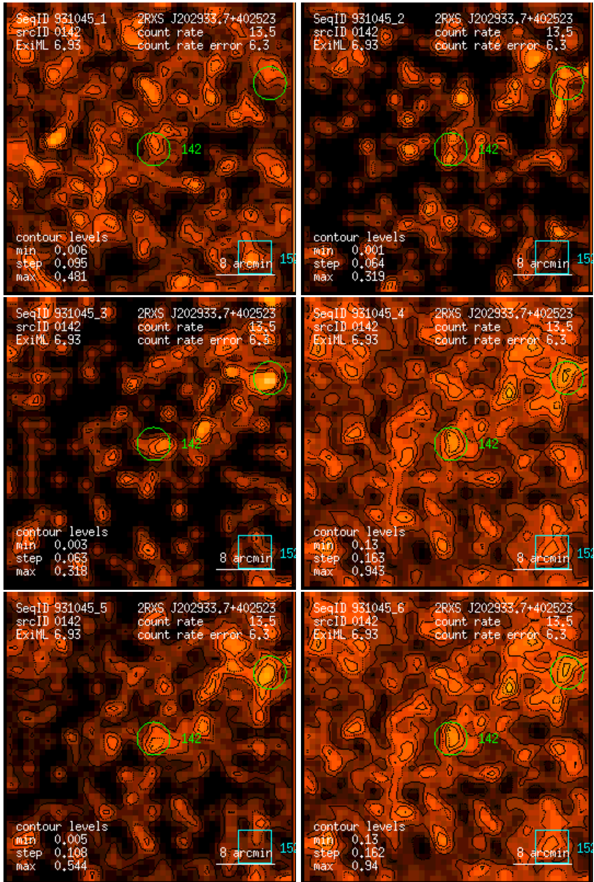
Figure 142: RASS 931045: detection 0142: band rate images, Gaussian filter: (1) PSPC channels 11 – 41, (2) 52 – 90, (3) 91 – 201, (4) 11 – 235, (5) 52 – 201, (6) 11 – 201. Broad band rates in counts/ks. Band rate contour levels in counts/ks/arcmin 2 .
