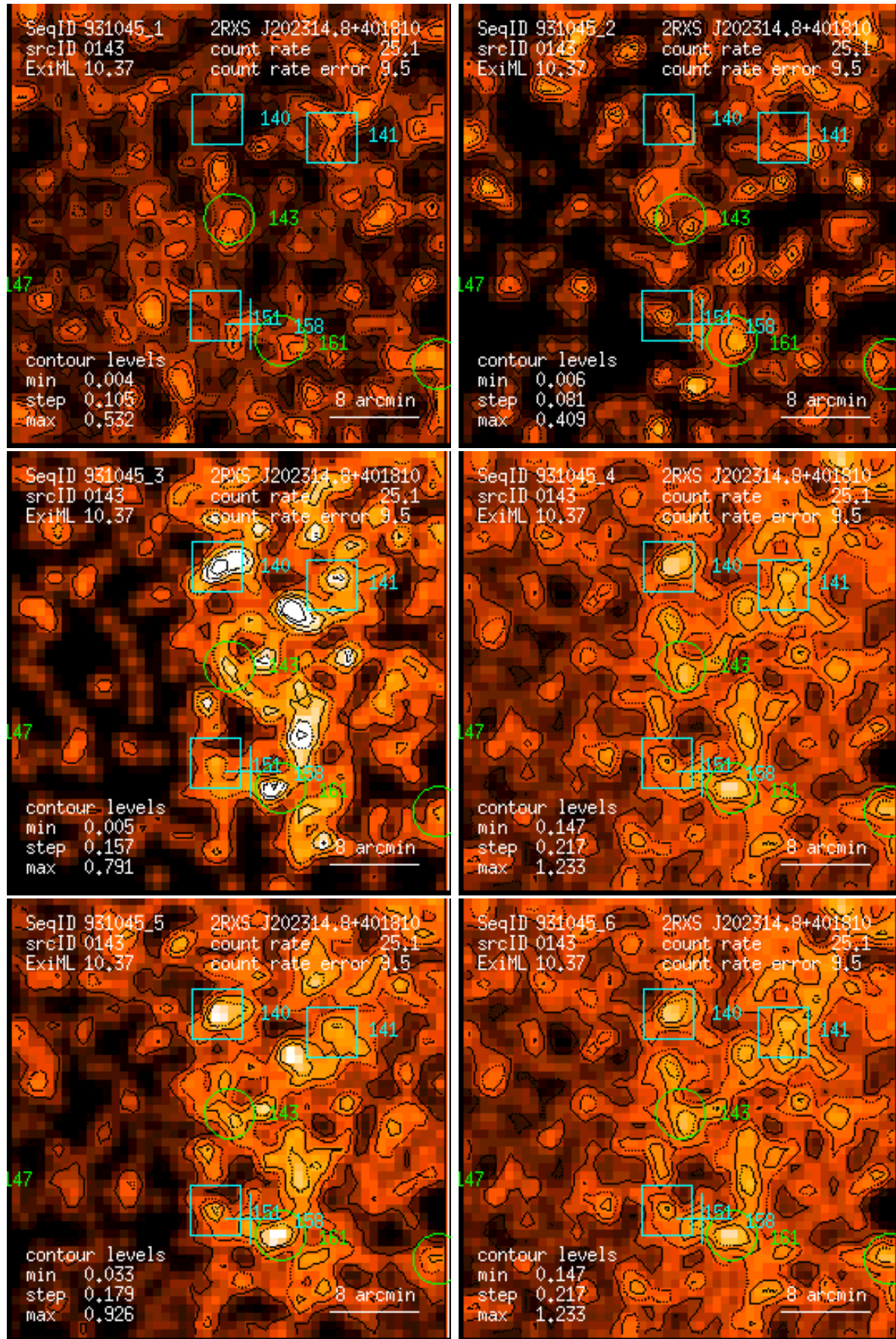
Figure 143: RASS 931045: detection 0143: band rate images, Gaussian filter: (1) PSPC channels 11 – 41, (2) 52 – 90, (3) 91 – 201, (4) 11 – 235, (5) 52 – 201, (6) 11 – 201. Broad band rates in counts/ks. Band rate contour levels in counts/ks/arcmin 2 .
