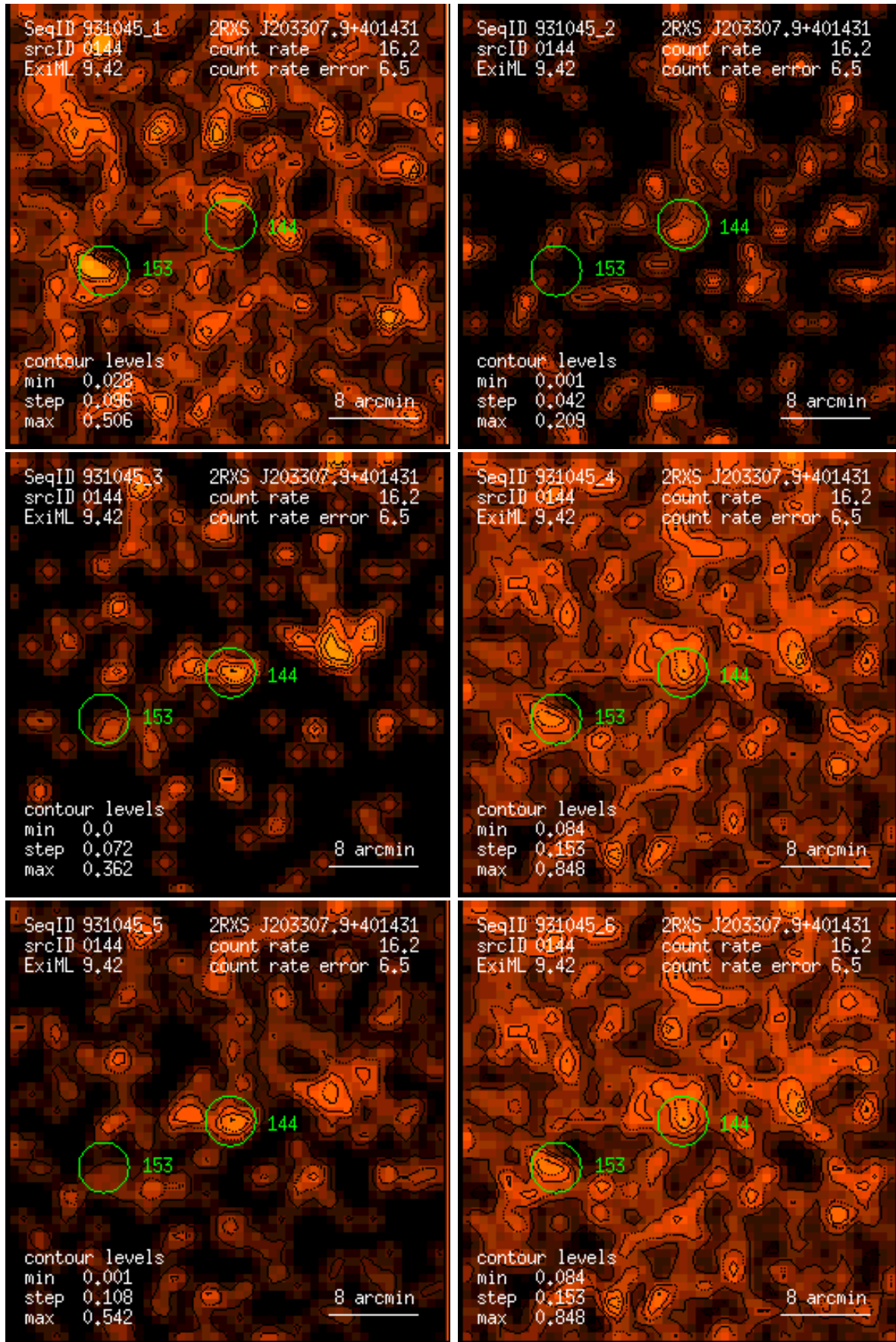
Figure 144: RASS 931045: detection 0144: band rate images, Gaussian filter: (1) PSPC channels 11 – 41, (2) 52 – 90, (3) 91 – 201, (4) 11 – 235, (5) 52 – 201, (6) 11 – 201. Broad band rates in counts/ks. Band rate contour levels in counts/ks/arcmin 2 .
