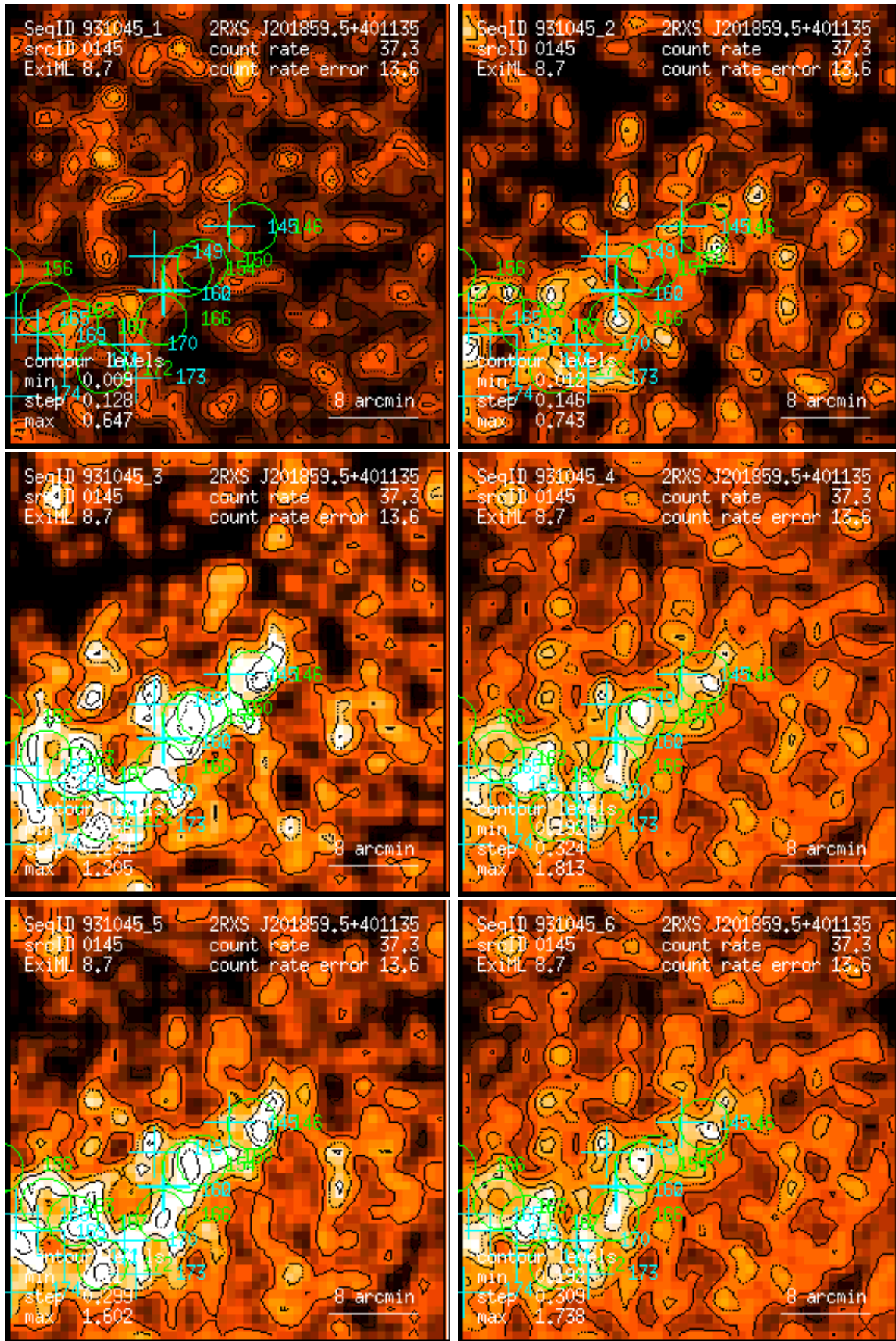
Figure 145: RASS 931045: detection 0145: band rate images, Gaussian filter: (1) PSPC channels 11 – 41, (2) 52 – 90, (3) 91 – 201, (4) 11 – 235, (5) 52 – 201, (6) 11 – 201. Broad band rates in counts/ks. Band rate contour levels in counts/ks/arcmin 2 .
