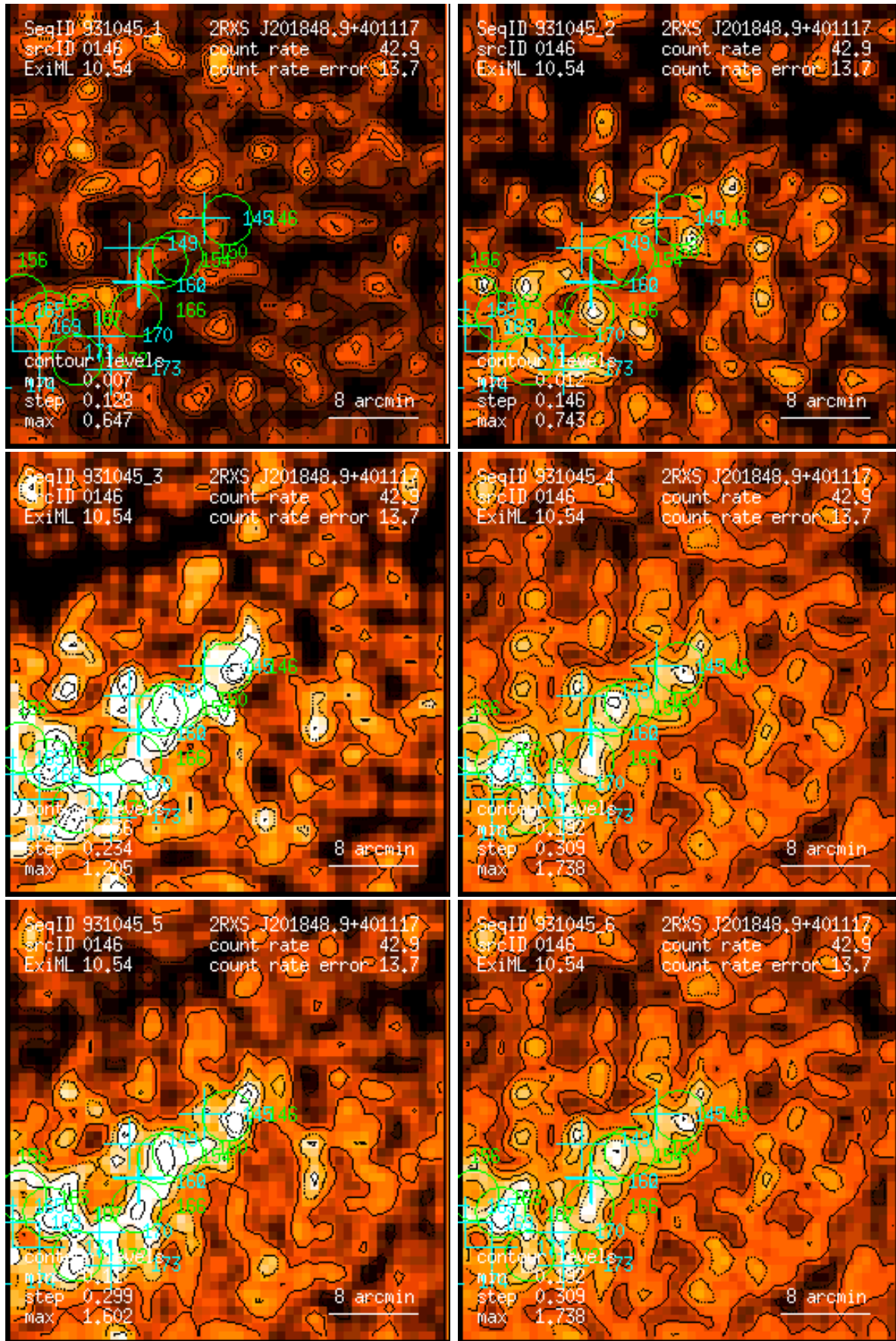
Figure 146: RASS 931045: detection 0146: band rate images, Gaussian filter: (1) PSPC channels 11 – 41, (2) 52 – 90, (3) 91 – 201, (4) 11 – 235, (5) 52 – 201, (6) 11 – 201. Broad band rates in counts/ks. Band rate contour levels in counts/ks/arcmin 2 .
