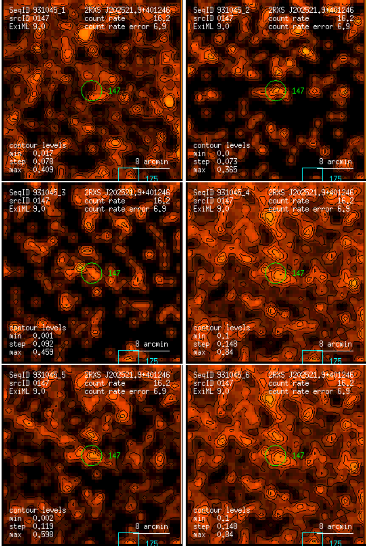
Figure 147: RASS 931045: detection 0147: band rate images, Gaussian filter: (1) PSPC channels 11 – 41, (2) 52 – 90, (3) 91 – 201, (4) 11 – 235, (5) 52 – 201, (6) 11 – 201. Broad band rates in counts/ks. Band rate contour levels in counts/ks/arcmin 2 .
