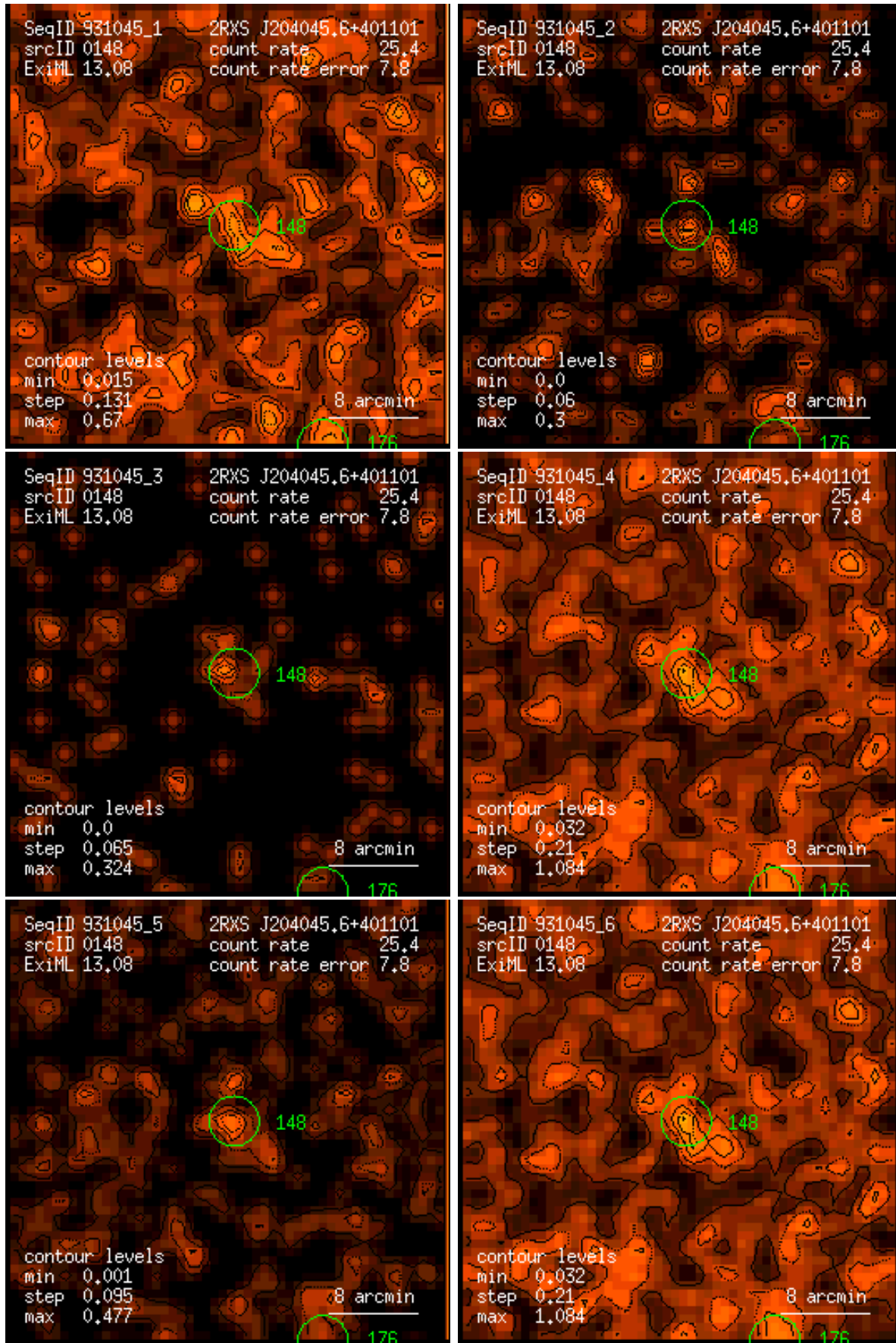
Figure 148: RASS 931045: detection 0148: band rate images, Gaussian filter: (1) PSPC channels 11 – 41, (2) 52 – 90, (3) 91 – 201, (4) 11 – 235, (5) 52 – 201, (6) 11 – 201. Broad band rates in counts/ks. Band rate contour levels in counts/ks/arcmin 2 .
