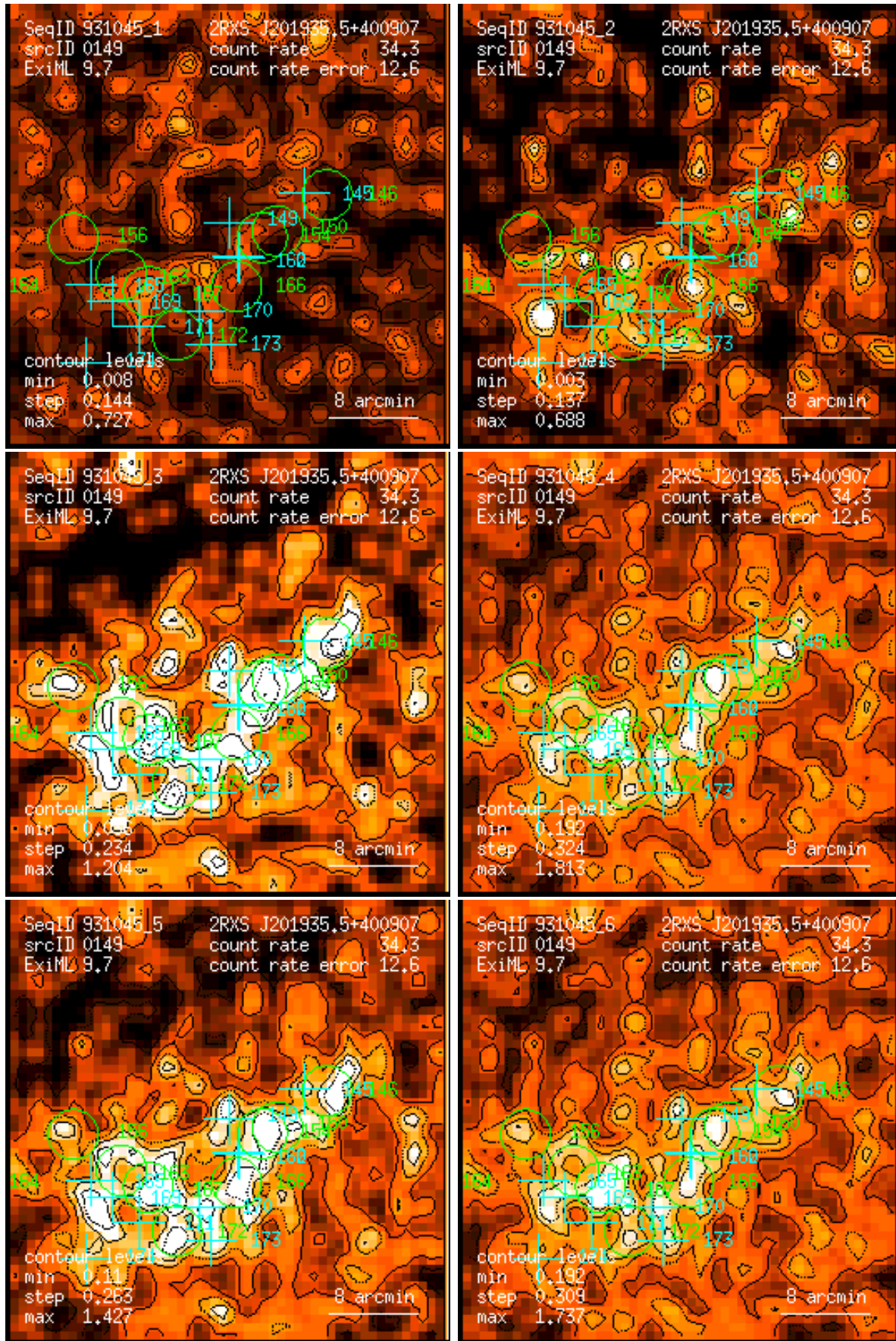
Figure 149: RASS 931045: detection 0149: band rate images, Gaussian filter: (1) PSPC channels 11 – 41, (2) 52 – 90, (3) 91 – 201, (4) 11 – 235, (5) 52 – 201, (6) 11 – 201. Broad band rates in counts/ks. Band rate contour levels in counts/ks/arcmin 2 .
