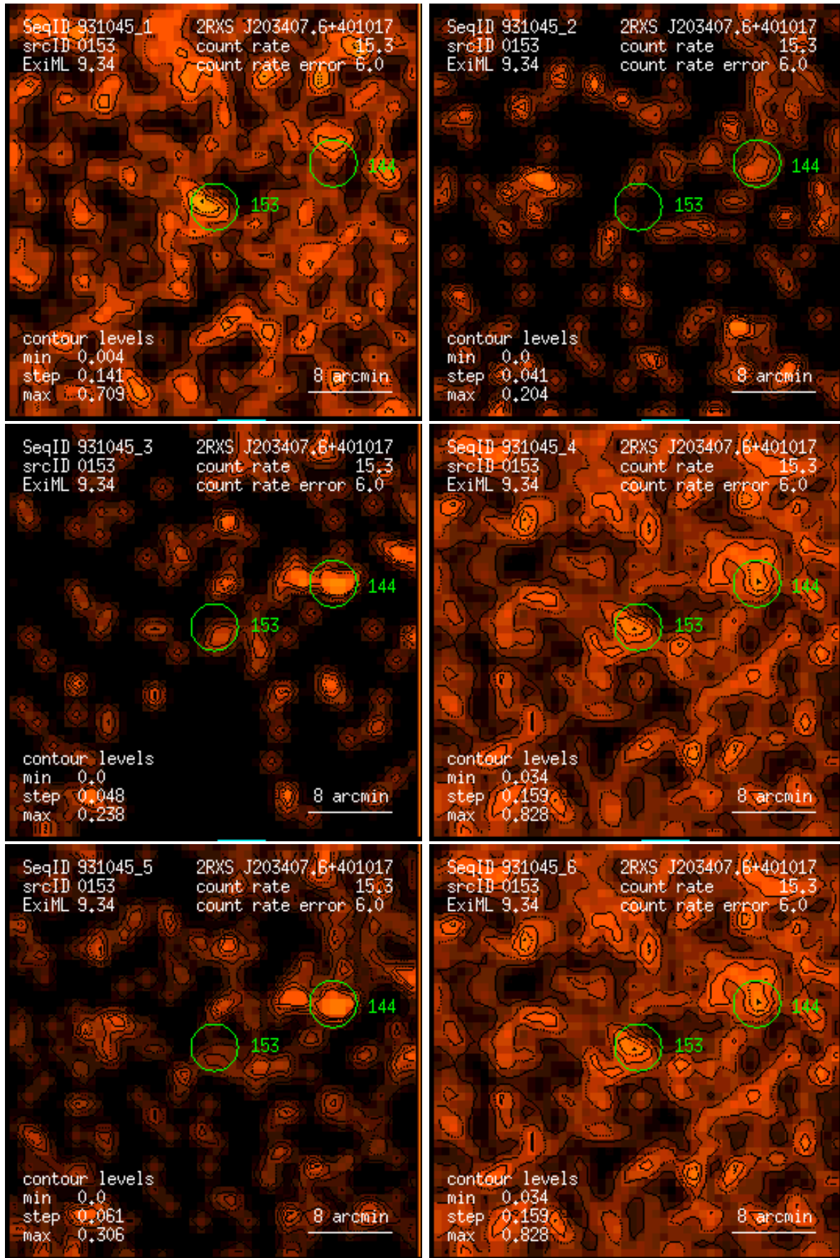
Figure 153: RASS 931045: detection 0153: band rate images, Gaussian filter: (1) PSPC channels 11 – 41, (2) 52 – 90, (3) 91 – 201, (4) 11 – 235, (5) 52 – 201, (6) 11 – 201. Broad band rates in counts/ks. Band rate contour levels in counts/ks/arcmin 2 .
