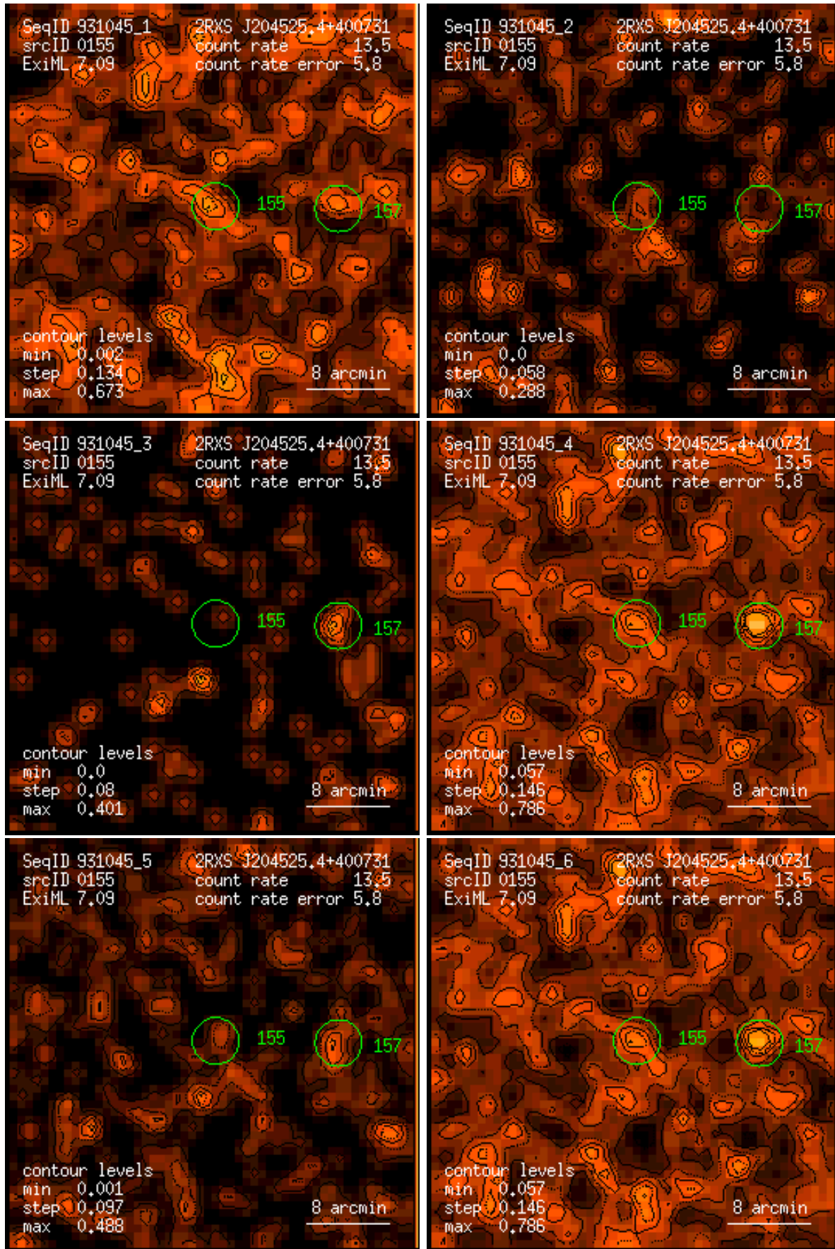
Figure 155: RASS 931045: detection 0155: band rate images, Gaussian filter: (1) PSPC channels 11 – 41, (2) 52 – 90, (3) 91 – 201, (4) 11 – 235, (5) 52 – 201, (6) 11 – 201. Broad band rates in counts/ks. Band rate contour levels in counts/ks/arcmin 2 .
