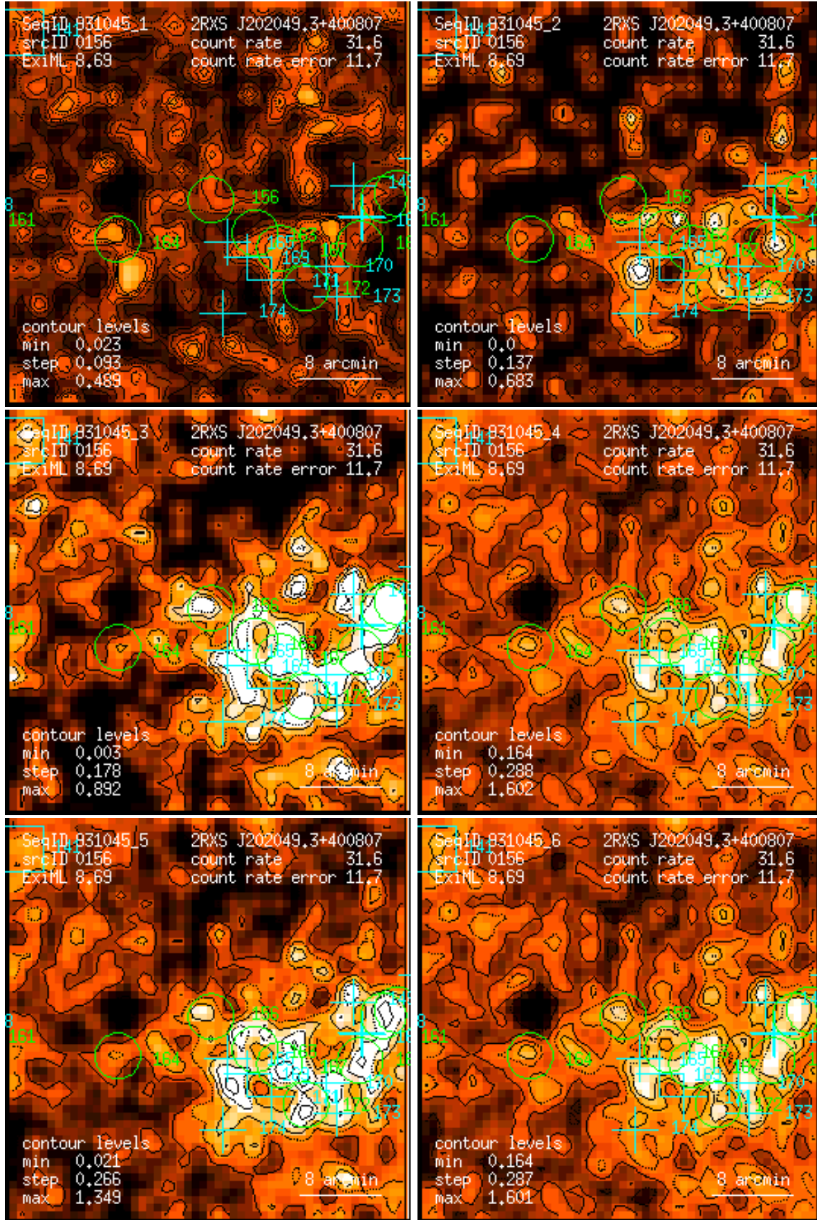
Figure 156: RASS 931045: detection 0156: band rate images, Gaussian filter: (1) PSPC channels 11 – 41, (2) 52 – 90, (3) 91 – 201, (4) 11 – 235, (5) 52 – 201, (6) 11 – 201. Broad band rates in counts/ks. Band rate contour levels in counts/ks/arcmin 2 .
