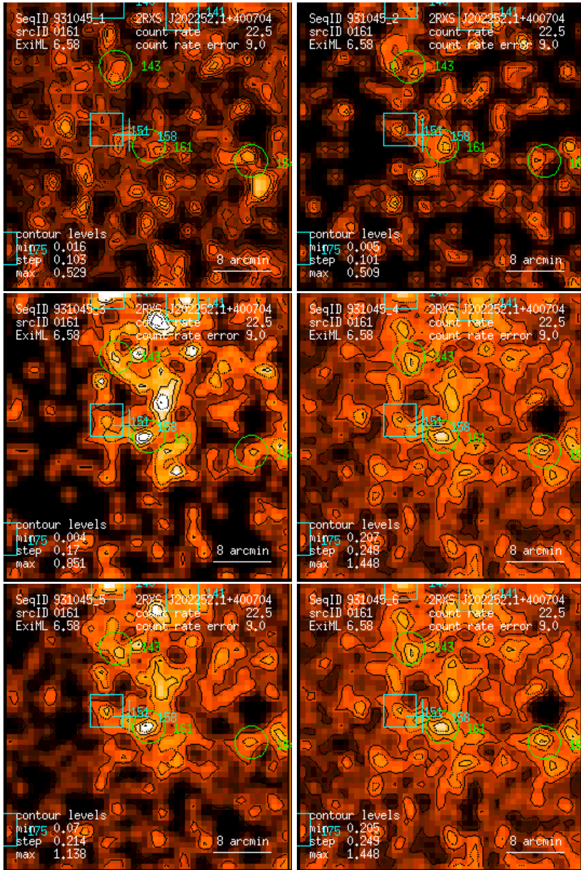
Figure 161: RASS 931045: detection 0161: band rate images, Gaussian filter: (1) PSPC channels 11 – 41, (2) 52 – 90, (3) 91 – 201, (4) 11 – 235, (5) 52 – 201, (6) 11 – 201. Broad band rates in counts/ks. Band rate contour levels in counts/ks/arcmin 2 .
