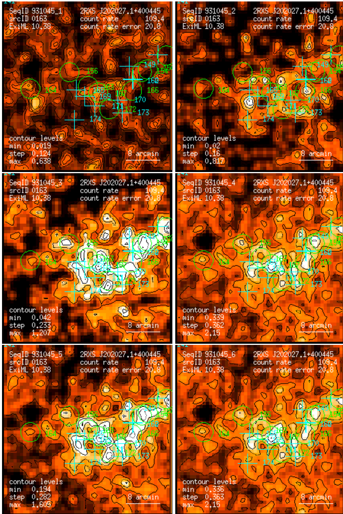
Figure 163: RASS 931045: detection 0163: band rate images, Gaussian filter: (1) PSPC channels 11 – 41, (2) 52 – 90, (3) 91 – 201, (4) 11 – 235, (5) 52 – 201, (6) 11 – 201. Broad band rates in counts/ks. Band rate contour levels in counts/ks/arcmin 2 .
