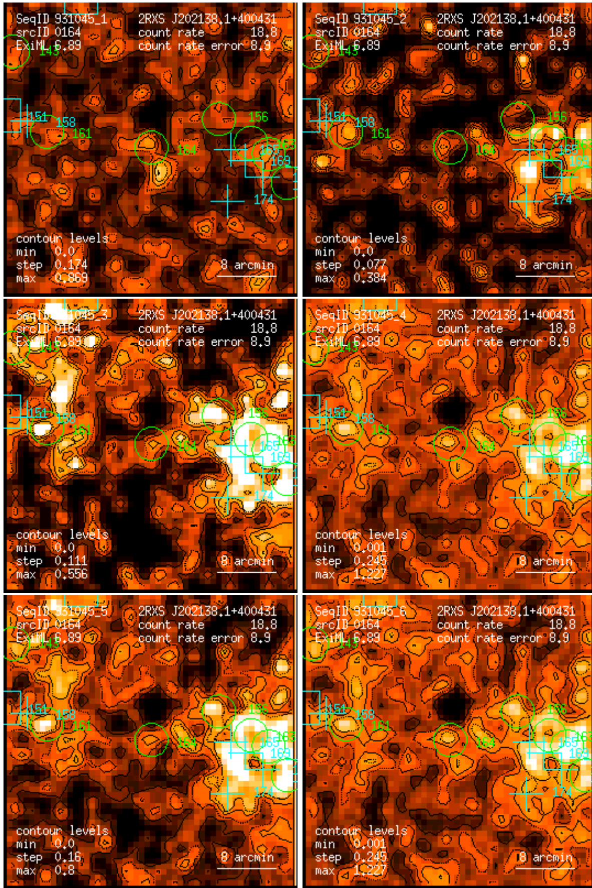
Figure 164: RASS 931045: detection 0164: band rate images, Gaussian filter: (1) PSPC channels 11 – 41, (2) 52 – 90, (3) 91 – 201, (4) 11 – 235, (5) 52 – 201, (6) 11 – 201. Broad band rates in counts/ks. Band rate contour levels in counts/ks/arcmin 2 .
