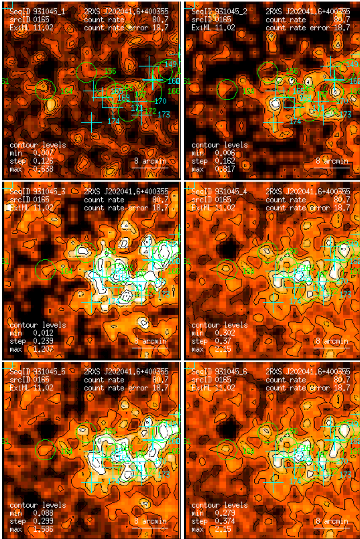
Figure 165: RASS 931045: detection 0165: band rate images, Gaussian filter: (1) PSPC channels 11 – 41, (2) 52 – 90, (3) 91 – 201, (4) 11 – 235, (5) 52 – 201, (6) 11 – 201. Broad band rates in counts/ks. Band rate contour levels in counts/ks/arcmin 2 .
